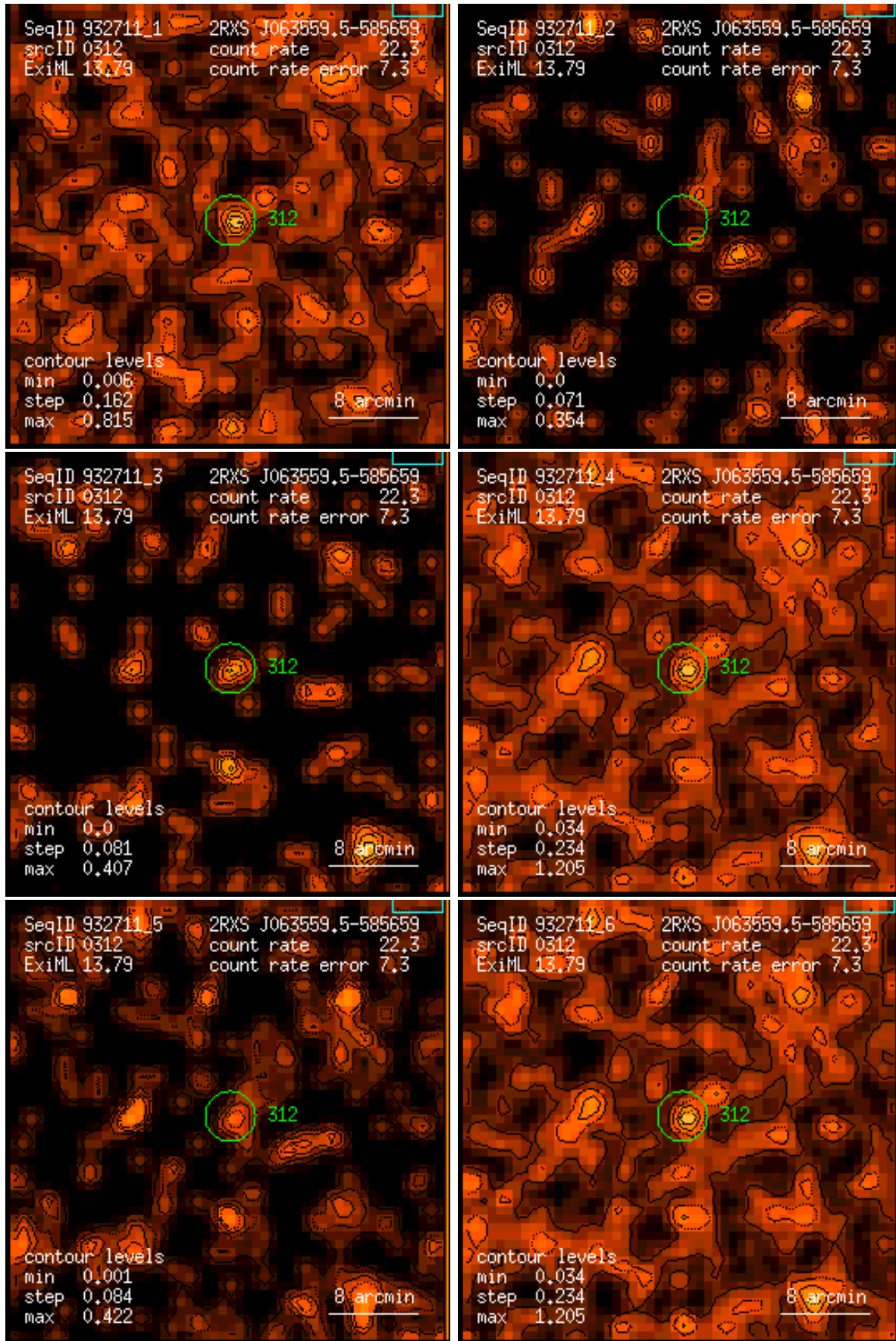
Figure 312: RASS 932711: detection 0312: band rate images, Gaussian filter: (1) PSPC channels 11 – 41, (2) 52 – 90, (3) 91 – 201, (4) 11 – 235, (5) 52 – 201, (6) 11 – 201. Broad band rates in counts/ks. Band rate contour levels in counts/ks/arcmin 2 .
