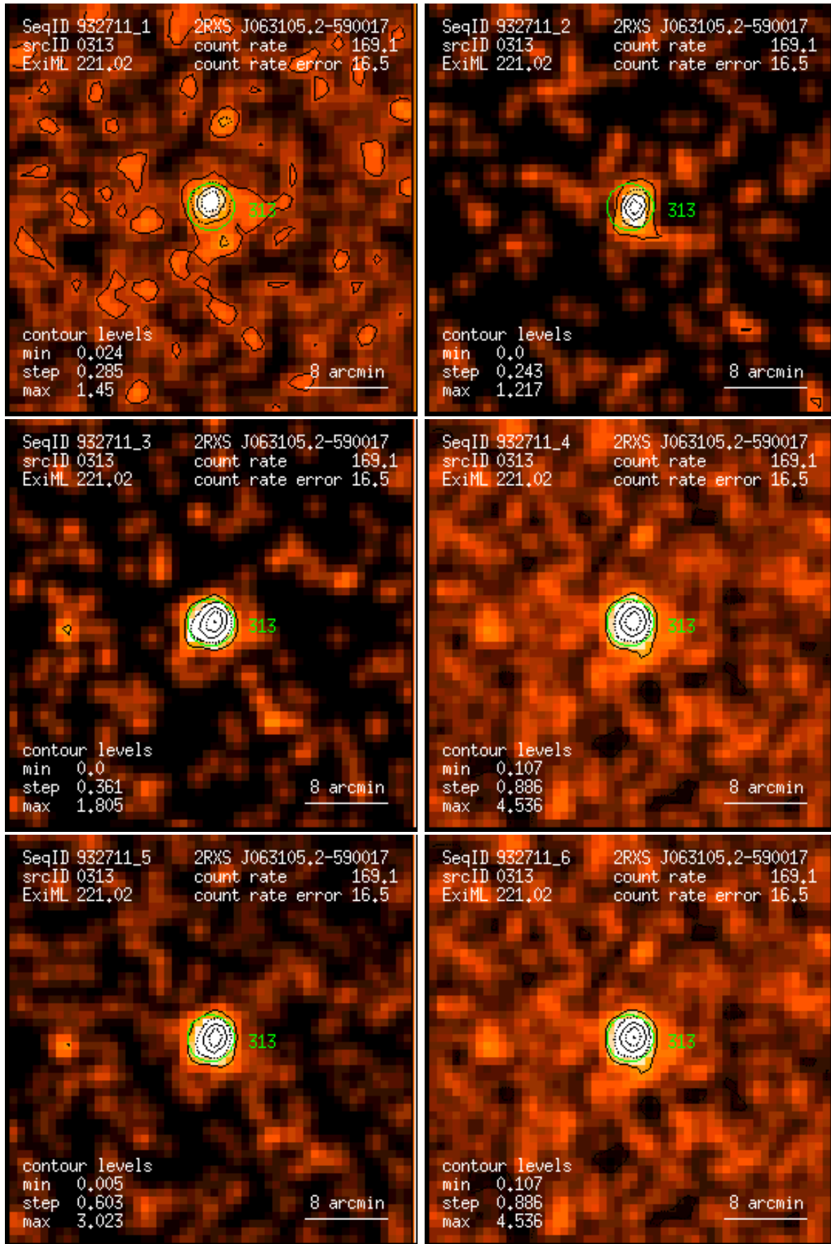
Figure 313: RASS 932711: detection 0313: band rate images, Gaussian filter: (1) PSPC channels 11 – 41, (2) 52 – 90, (3) 91 – 201, (4) 11 – 235, (5) 52 – 201, (6) 11 – 201. Broad band rates in counts/ks. Band rate contour levels in counts/ks/arcmin 2 .
