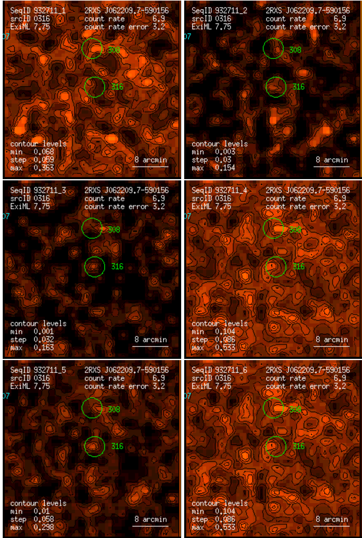
Figure 316: RASS 932711: detection 0316: band rate images, Gaussian filter: (1) PSPC channels 11 – 41, (2) 52 – 90, (3) 91 – 201, (4) 11 – 235, (5) 52 – 201, (6) 11 – 201. Broad band rates in counts/ks. Band rate contour levels in counts/ks/arcmin 2 .
