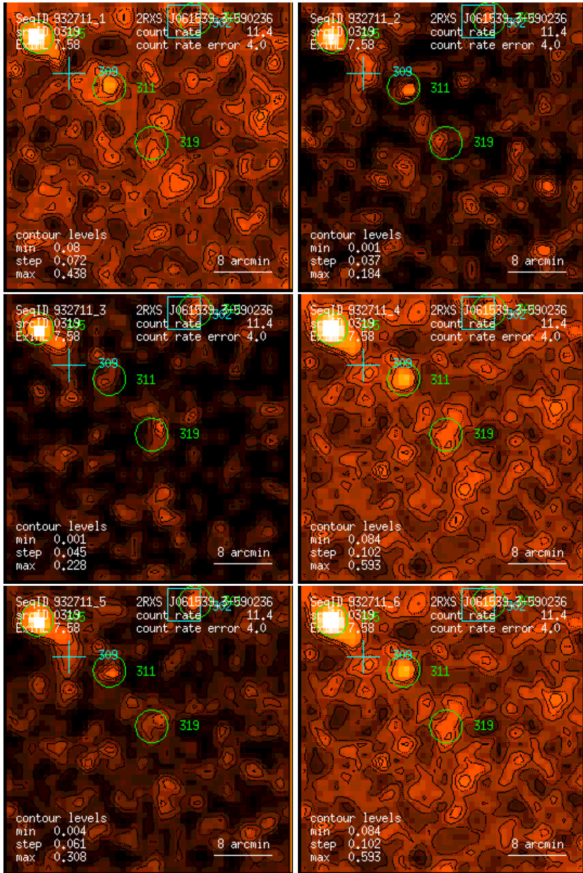
Figure 319: RASS 932711: detection 0319: band rate images, Gaussian filter: (1) PSPC channels 11 – 41, (2) 52 – 90, (3) 91 – 201, (4) 11 – 235, (5) 52 – 201, (6) 11 – 201. Broad band rates in counts/ks. Band rate contour levels in counts/ks/arcmin 2 .
