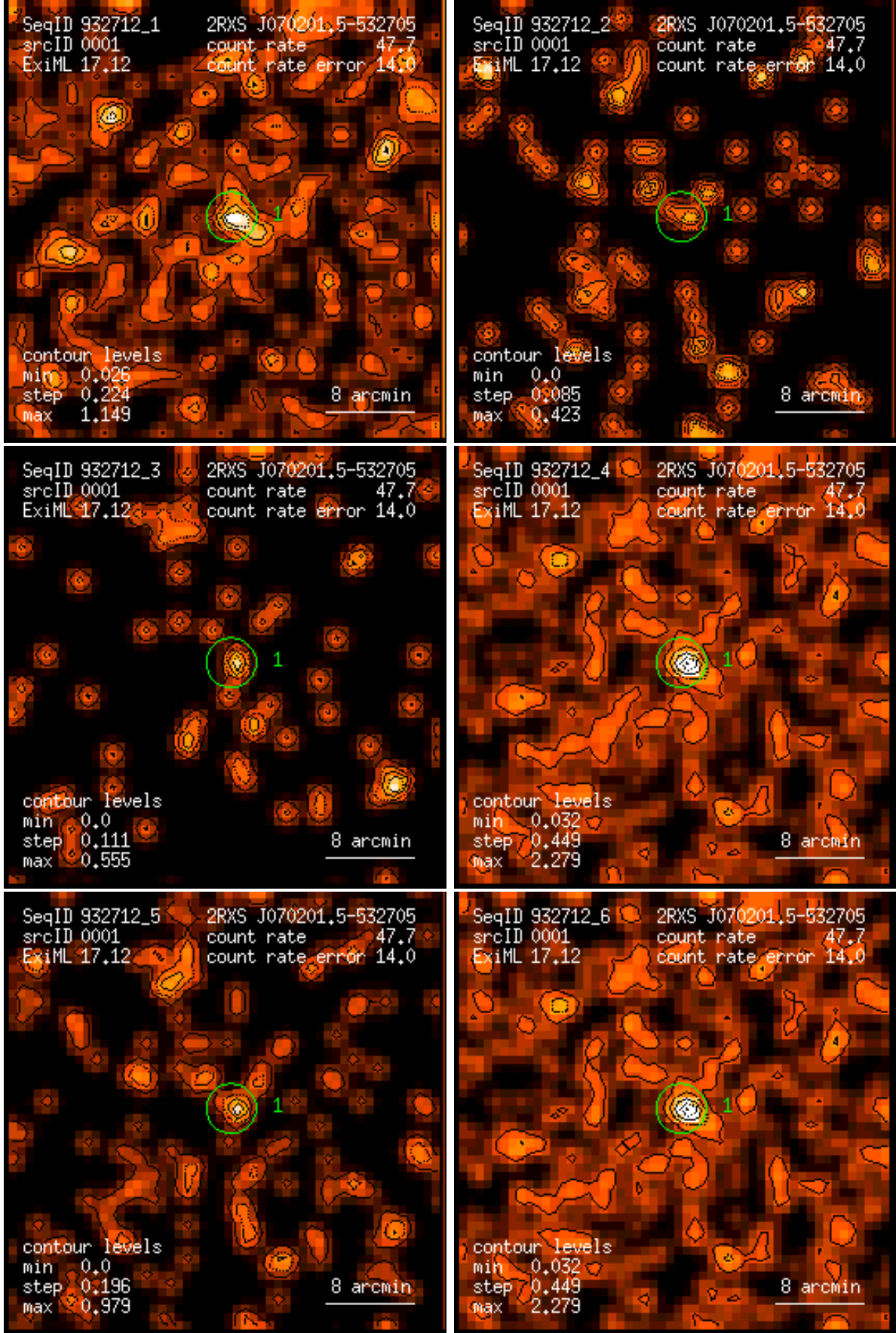
Figure 1: RASS 932712: detection 0001: band rate images, Gaussian filter: (1) PSPC channels 11 – 41, (2) 52 – 90, (3) 91 – 201, (4) 11 – 235, (5) 52 – 201, (6) 11 – 201. Broad band rates in counts/ks. Band rate contour levels in counts/ks/arcmin 2 .
