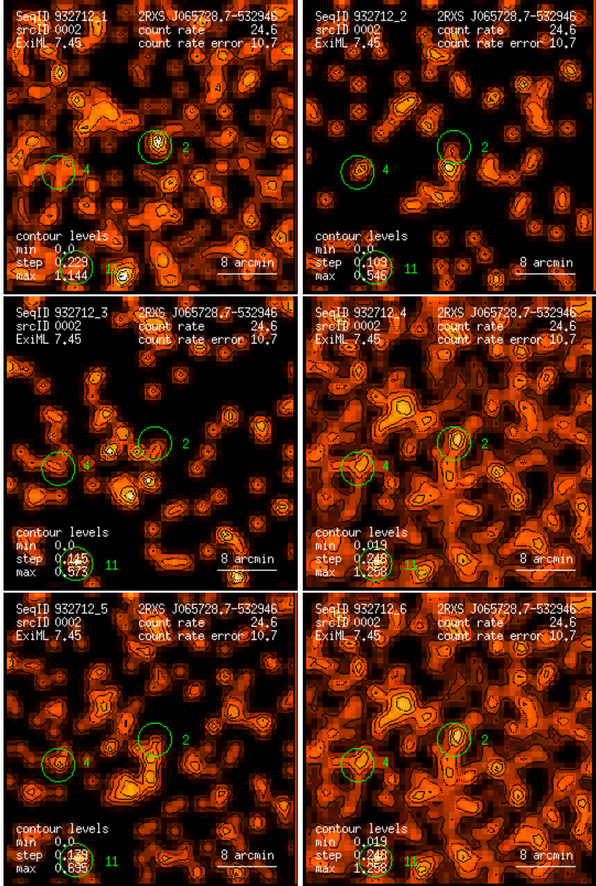
Figure 2: RASS 932712: detection 0002: band rate images, Gaussian filter: (1) PSPC channels 11 – 41, (2) 52 – 90, (3) 91 – 201, (4) 11 – 235, (5) 52 – 201, (6) 11 – 201. Broad band rates in counts/ks. Band rate contour levels in counts/ks/arcmin 2 .
