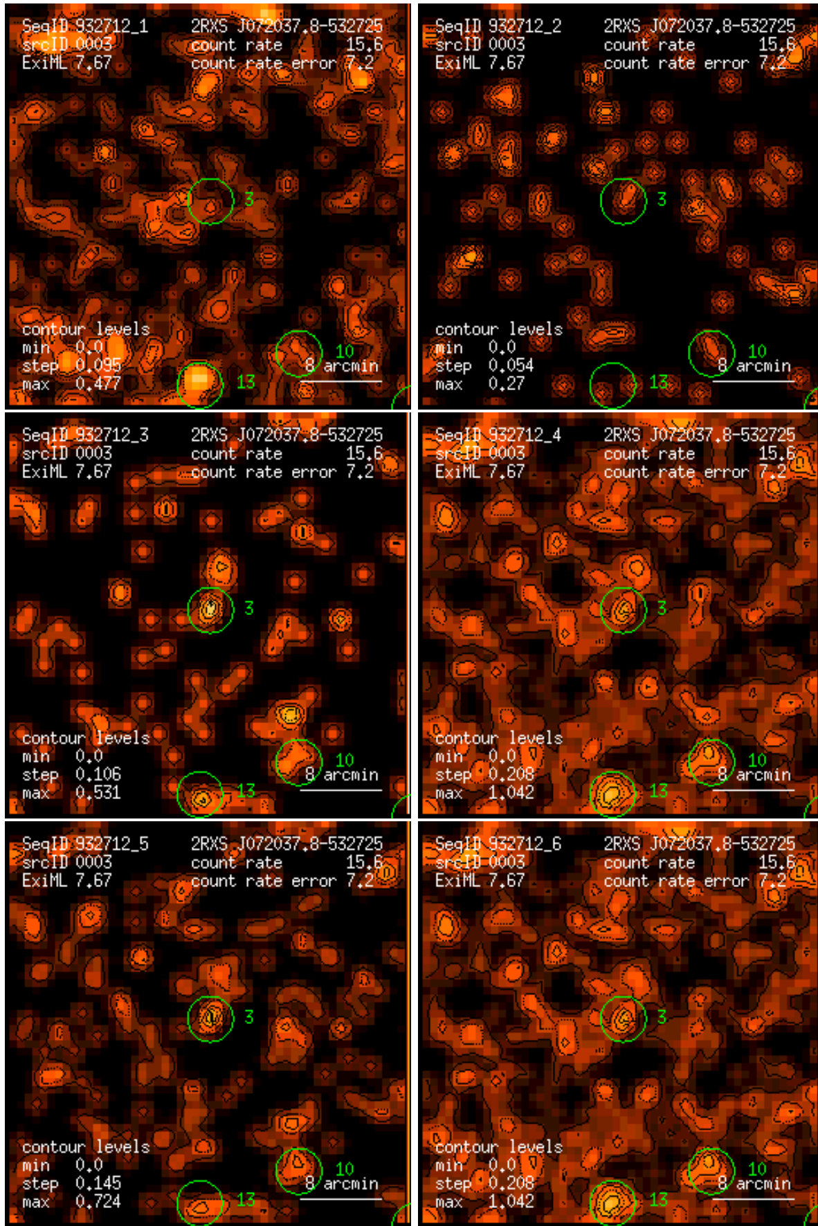
Figure 3: RASS 932712: detection 0003: band rate images, Gaussian filter: (1) PSPC channels 11 – 41, (2) 52 – 90, (3) 91 – 201, (4) 11 – 235, (5) 52 – 201, (6) 11 – 201. Broad band rates in counts/ks. Band rate contour levels in counts/ks/arcmin 2 .
