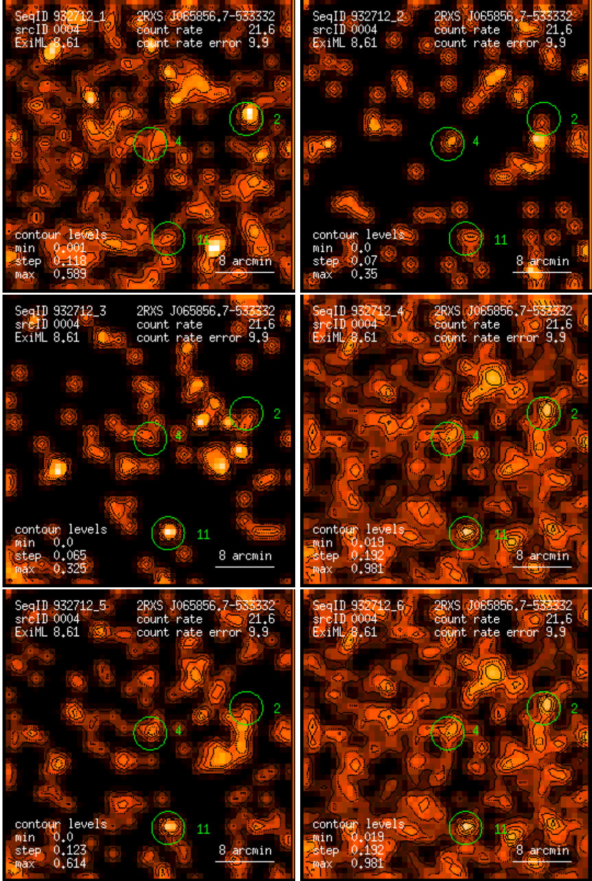
Figure 4: RASS 932712: detection 0004: band rate images, Gaussian filter: (1) PSPC channels 11 – 41, (2) 52 – 90, (3) 91 – 201, (4) 11 – 235, (5) 52 – 201, (6) 11 – 201. Broad band rates in counts/ks. Band rate contour levels in counts/ks/arcmin 2 .
