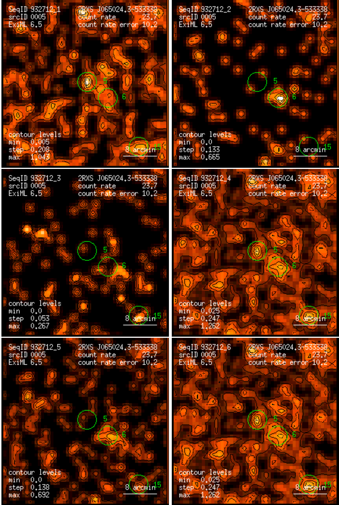
Figure 5: RASS 932712: detection 0005: band rate images, Gaussian filter: (1) PSPC channels 11 – 41, (2) 52 – 90, (3) 91 – 201, (4) 11 – 235, (5) 52 – 201, (6) 11 – 201. Broad band rates in counts/ks. Band rate contour levels in counts/ks/arcmin 2 .
