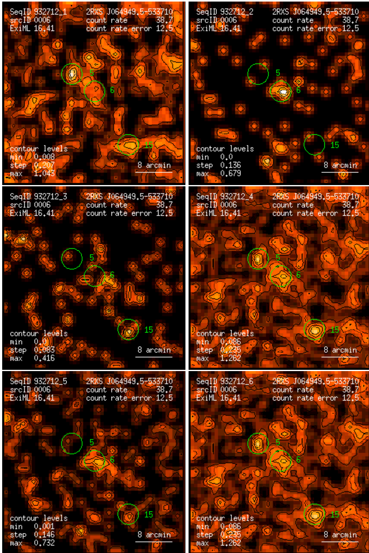
Figure 6: RASS 932712: detection 0006: band rate images, Gaussian filter: (1) PSPC channels 11 – 41, (2) 52 – 90, (3) 91 – 201, (4) 11 – 235, (5) 52 – 201, (6) 11 – 201. Broad band rates in counts/ks. Band rate contour levels in counts/ks/arcmin 2 .
