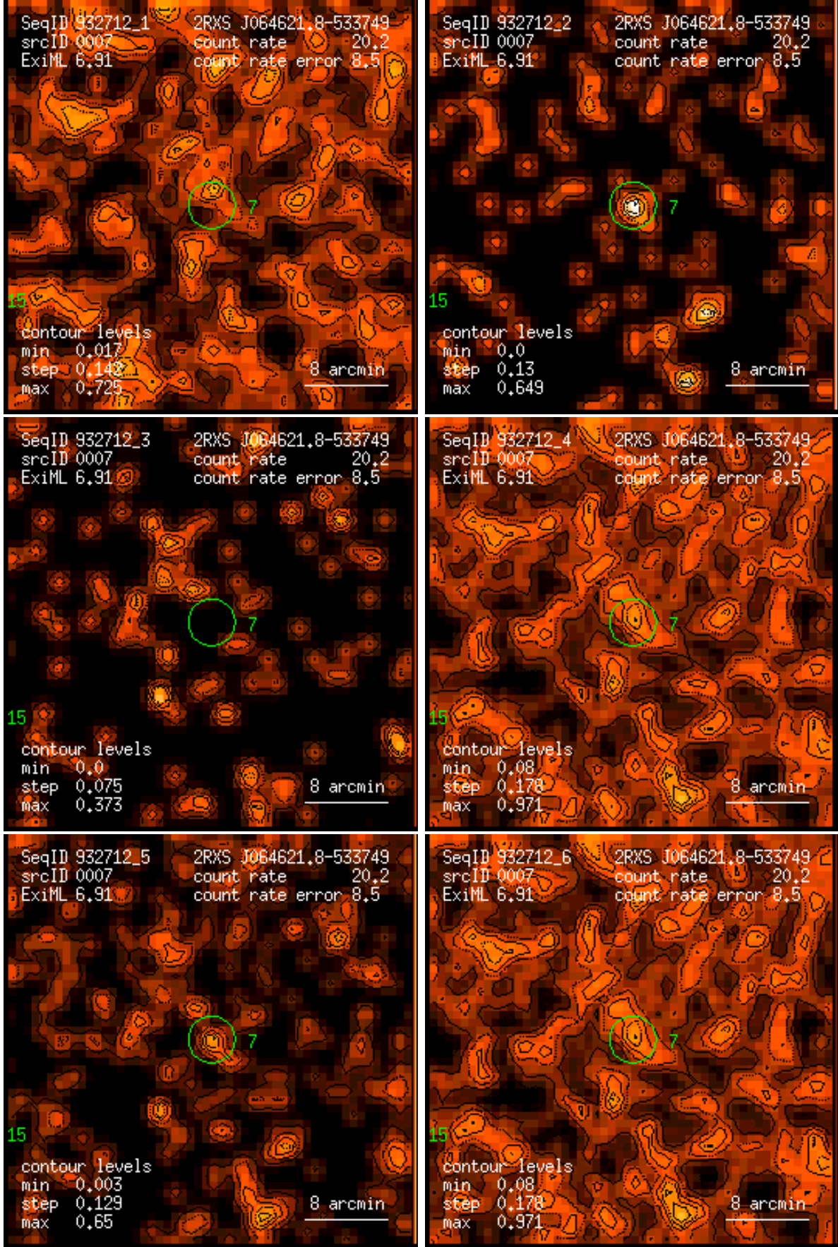
Figure 7: RASS 932712: detection 0007: band rate images, Gaussian filter: (1) PSPC channels 11 – 41, (2) 52 – 90, (3) 91 – 201, (4) 11 – 235, (5) 52 – 201, (6) 11 – 201. Broad band rates in counts/ks. Band rate contour levels in counts/ks/arcmin 2 .
