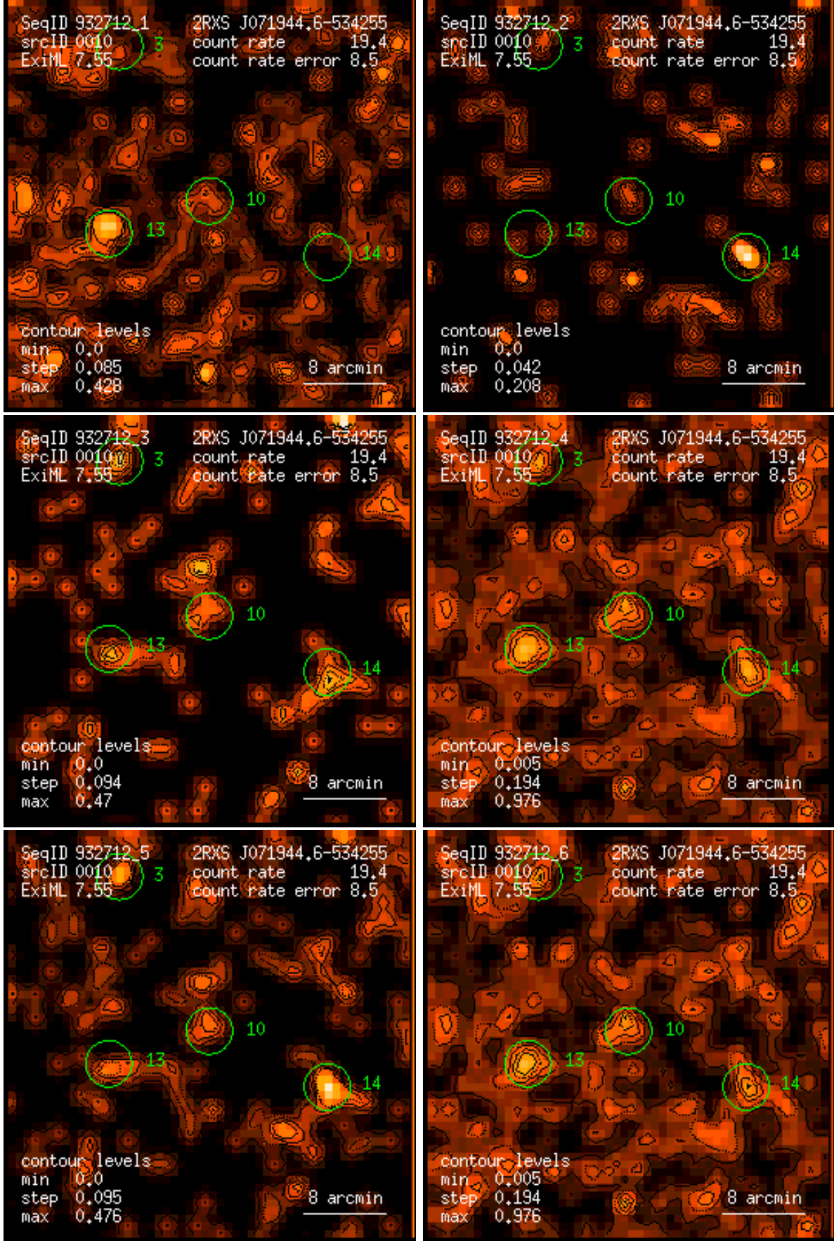
Figure 10: RASS 932712: detection 0010: band rate images, Gaussian filter: (1) PSPC channels 11 – 41, (2) 52 – 90, (3) 91 – 201, (4) 11 – 235, (5) 52 – 201, (6) 11 – 201. Broad band rates in counts/ks. Band rate contour levels in counts/ks/arcmin 2 .
