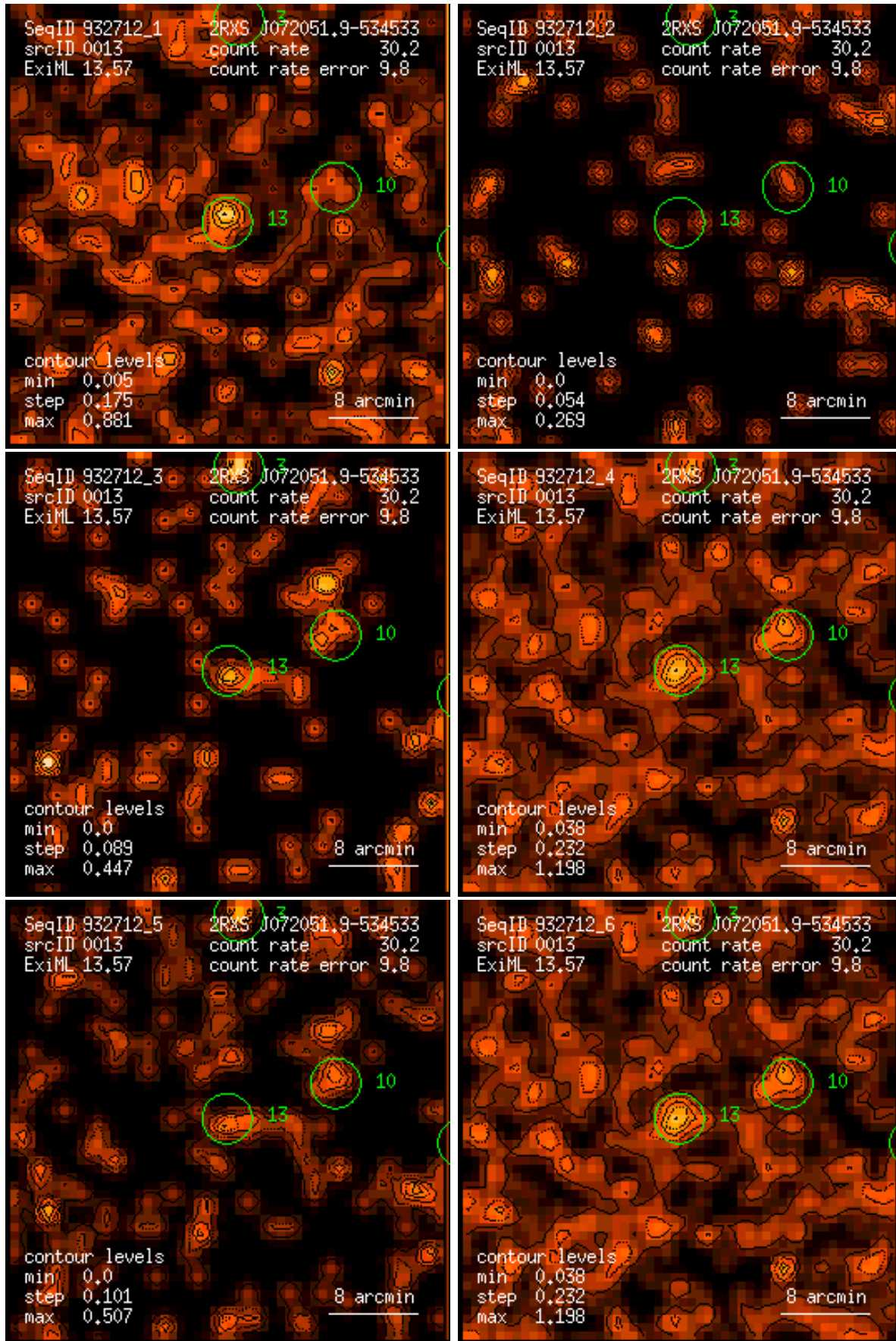
Figure 13: RASS 932712: detection 0013: band rate images, Gaussian filter: (1) PSPC channels 11 – 41, (2) 52 – 90, (3) 91 – 201, (4) 11 – 235, (5) 52 – 201, (6) 11 – 201. Broad band rates in counts/ks. Band rate contour levels in counts/ks/arcmin 2 .
