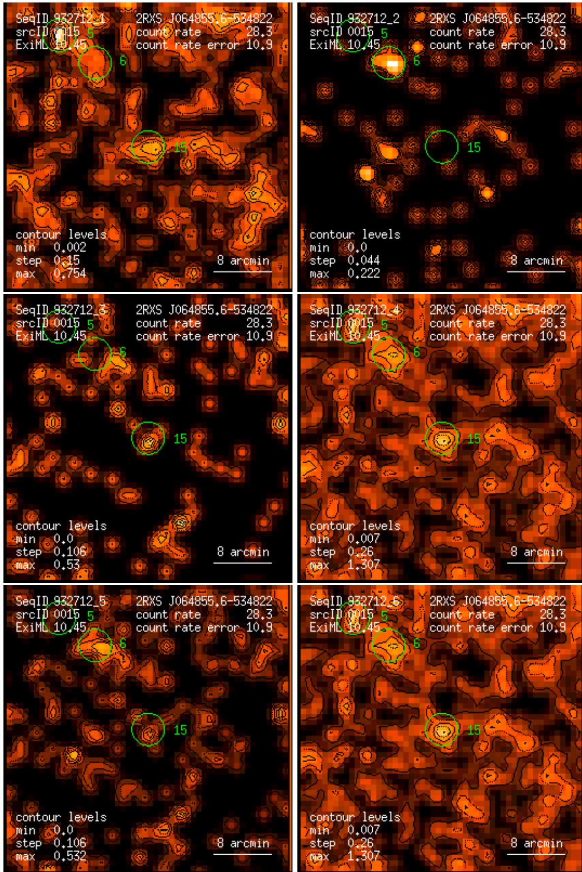
Figure 15: RASS 932712: detection 0015: band rate images, Gaussian filter: (1) PSPC channels 11 – 41, (2) 52 – 90, (3) 91 – 201, (4) 11 – 235, (5) 52 – 201, (6) 11 – 201. Broad band rates in counts/ks. Band rate contour levels in counts/ks/arcmin 2 .
