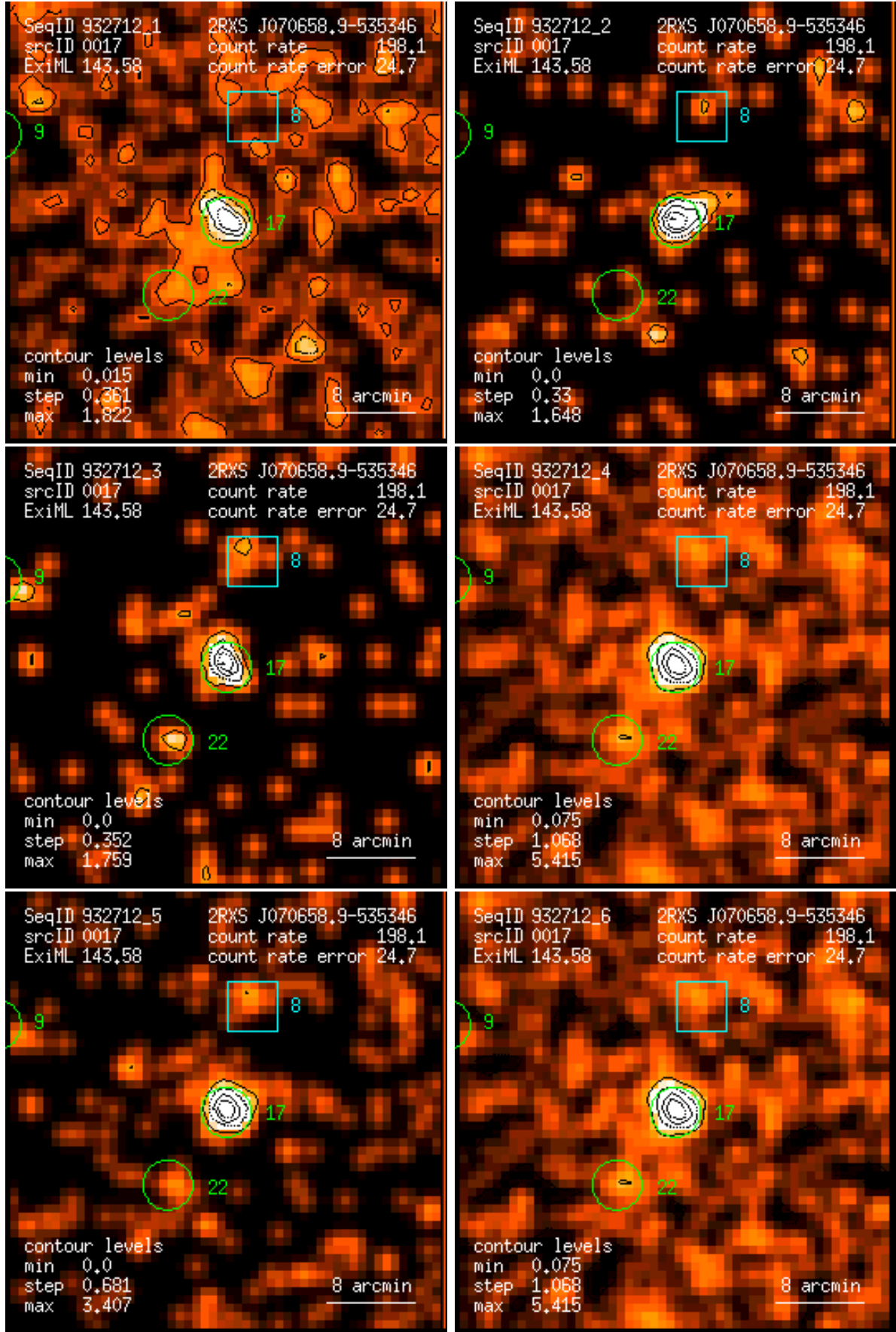
Figure 17: RASS 932712: detection 0017: band rate images, Gaussian filter: (1) PSPC channels 11 – 41, (2) 52 – 90, (3) 91 – 201, (4) 11 – 235, (5) 52 – 201, (6) 11 – 201. Broad band rates in counts/ks. Band rate contour levels in counts/ks/arcmin 2 .
