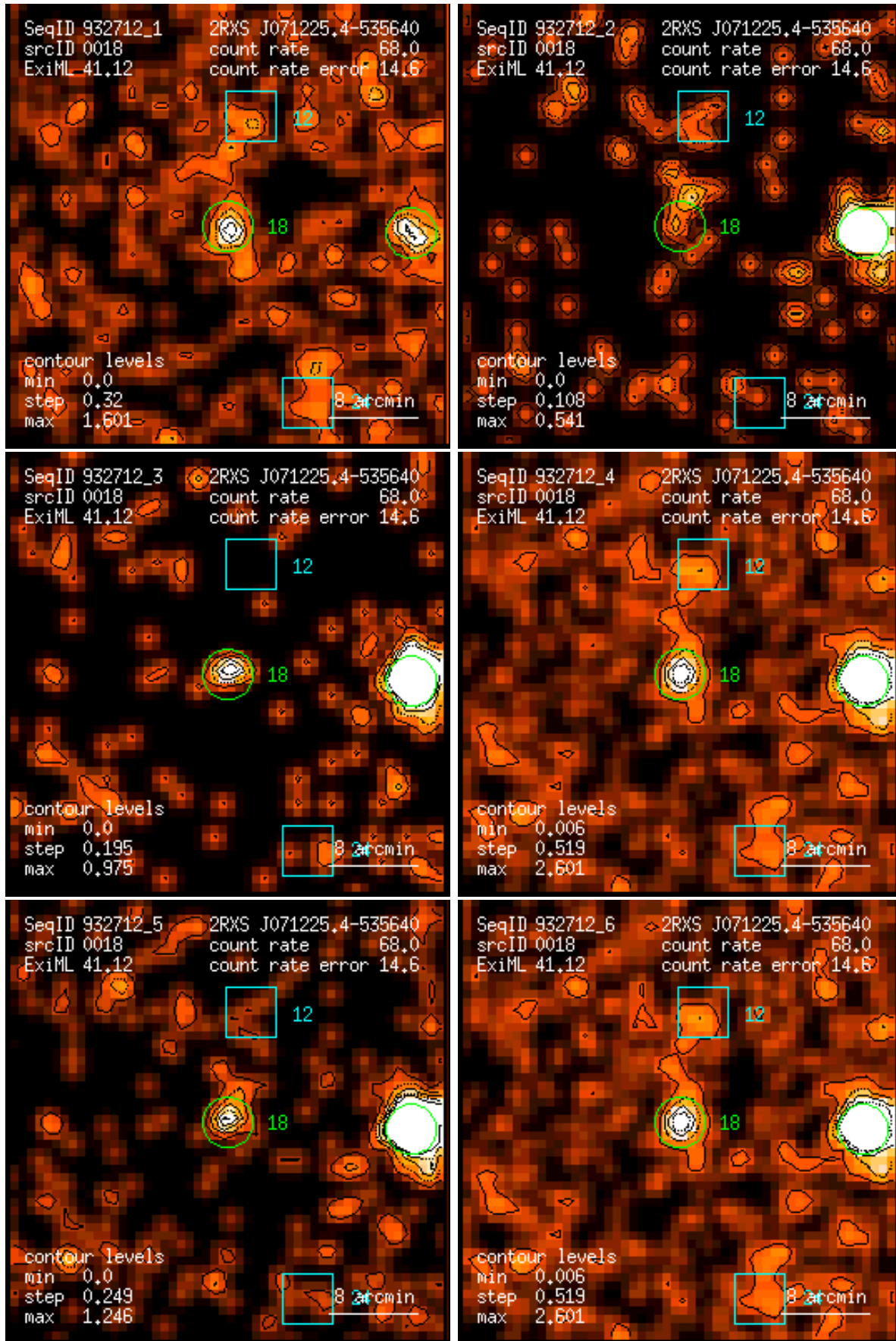
Figure 18: RASS 932712: detection 0018: band rate images, Gaussian filter: (1) PSPC channels 11 – 41, (2) 52 – 90, (3) 91 – 201, (4) 11 – 235, (5) 52 – 201, (6) 11 – 201. Broad band rates in counts/ks. Band rate contour levels in counts/ks/arcmin 2 .
