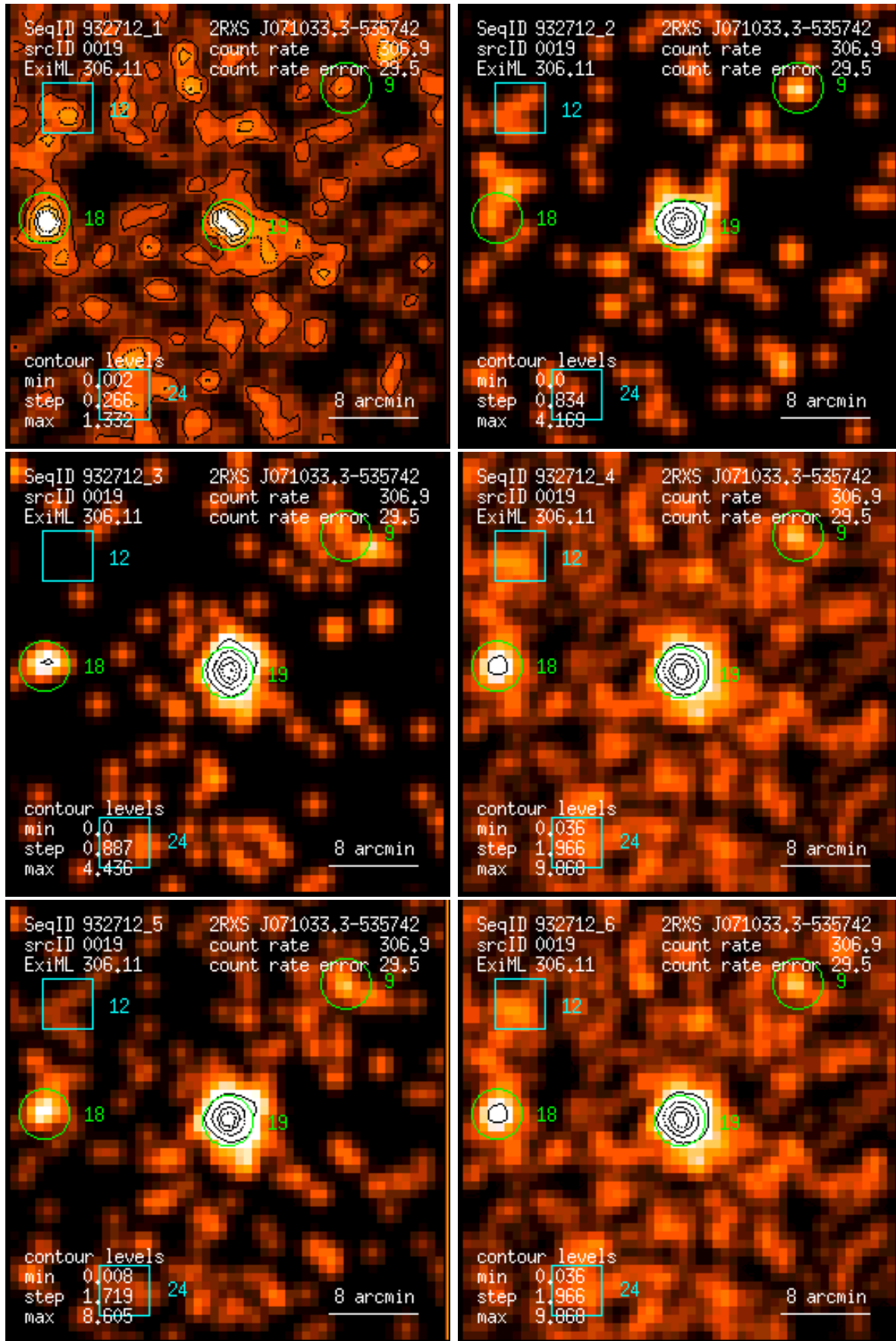
Figure 19: RASS 932712: detection 0019: band rate images, Gaussian filter: (1) PSPC channels 11 – 41, (2) 52 – 90, (3) 91 – 201, (4) 11 – 235, (5) 52 – 201, (6) 11 – 201. Broad band rates in counts/ks. Band rate contour levels in counts/ks/arcmin 2 .
