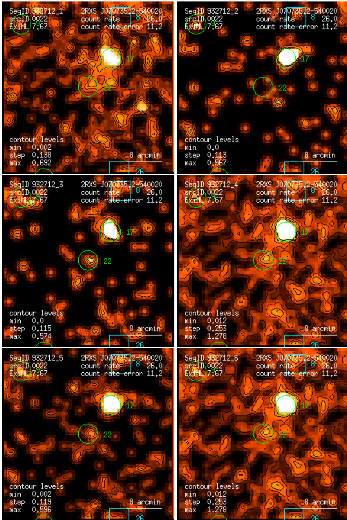
Figure 22: RASS 932712: detection 0022: band rate images, Gaussian filter: (1) PSPC channels 11 – 41, (2) 52 – 90, (3) 91 – 201, (4) 11 – 235, (5) 52 – 201, (6) 11 – 201. Broad band rates in counts/ks. Band rate contour levels in counts/ks/arcmin 2 .
