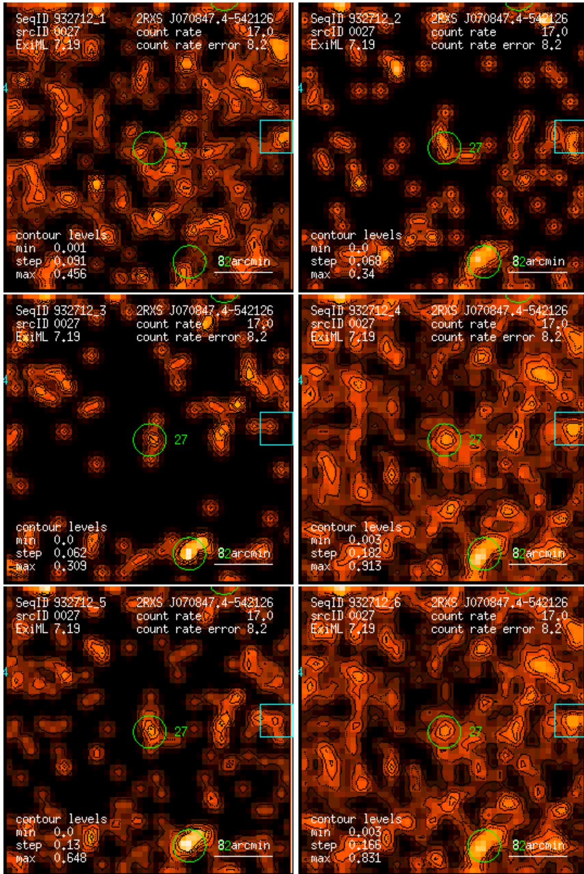
Figure 27: RASS 932712: detection 0027: band rate images, Gaussian filter: (1) PSPC channels 11 – 41, (2) 52 – 90, (3) 91 – 201, (4) 11 – 235, (5) 52 – 201, (6) 11 – 201. Broad band rates in counts/ks. Band rate contour levels in counts/ks/arcmin 2 .
