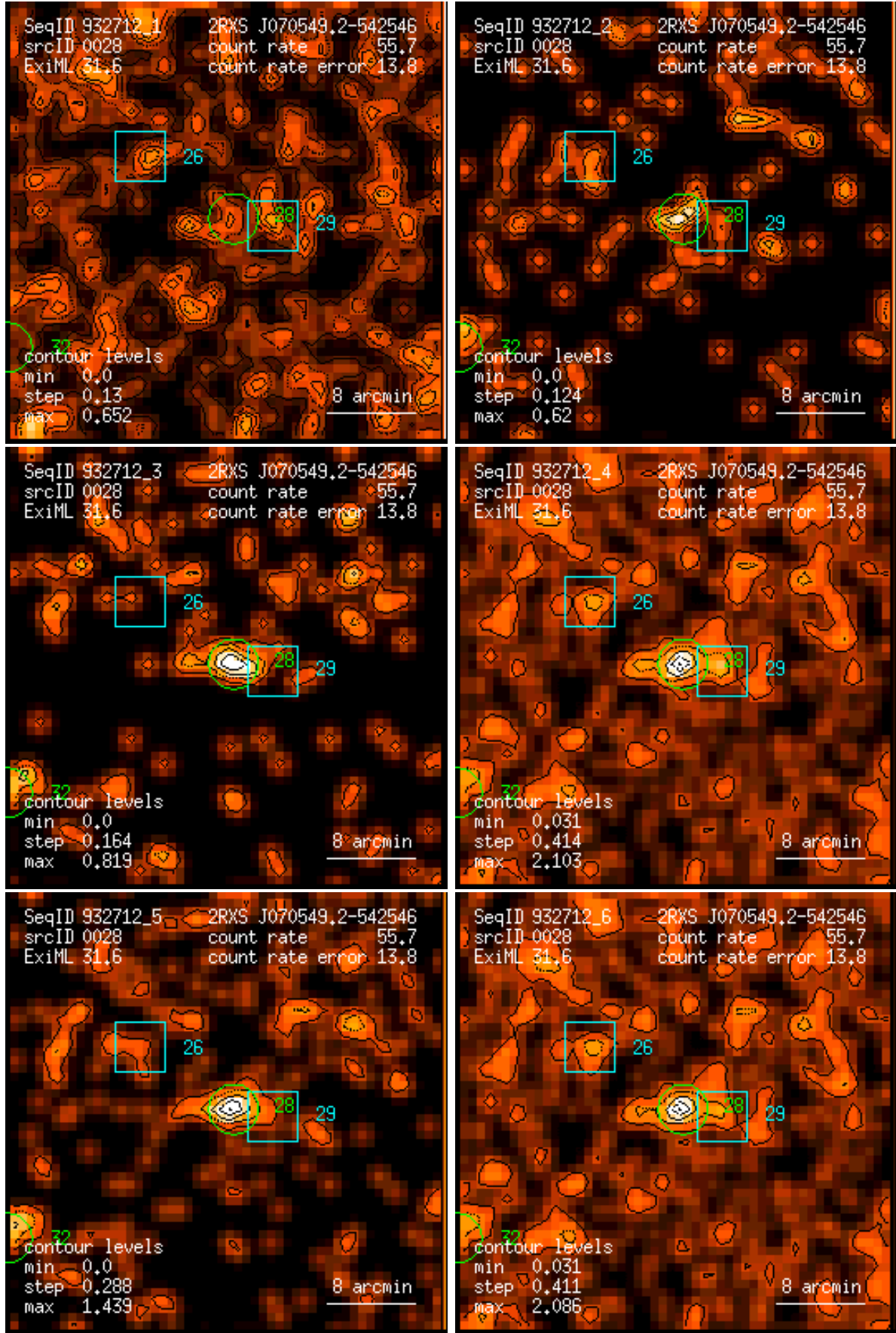
Figure 28: RASS 932712: detection 0028: band rate images, Gaussian filter: (1) PSPC channels 11 – 41, (2) 52 – 90, (3) 91 – 201, (4) 11 – 235, (5) 52 – 201, (6) 11 – 201. Broad band rates in counts/ks. Band rate contour levels in counts/ks/arcmin 2 .
