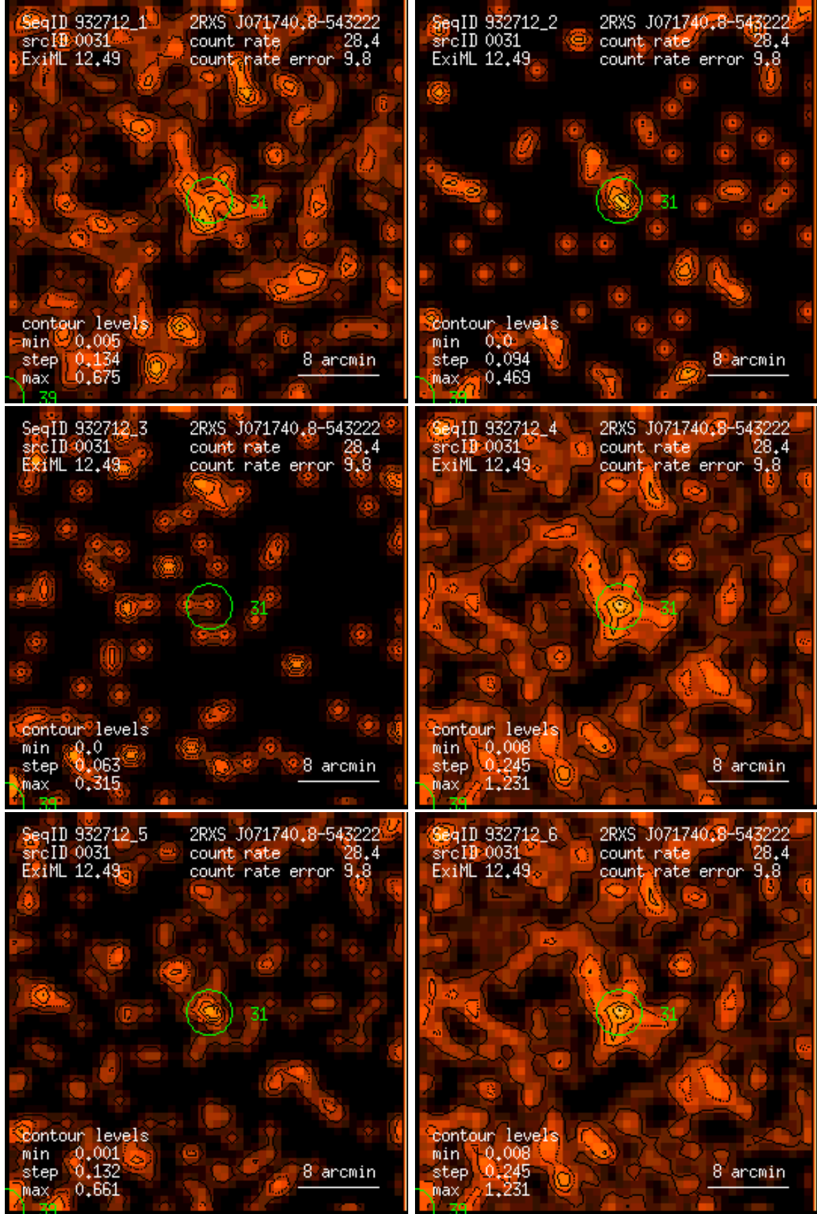
Figure 31: RASS 932712: detection 0031: band rate images, Gaussian filter: (1) PSPC channels 11 – 41, (2) 52 – 90, (3) 91 – 201, (4) 11 – 235, (5) 52 – 201, (6) 11 – 201. Broad band rates in counts/ks. Band rate contour levels in counts/ks/arcmin 2 .
