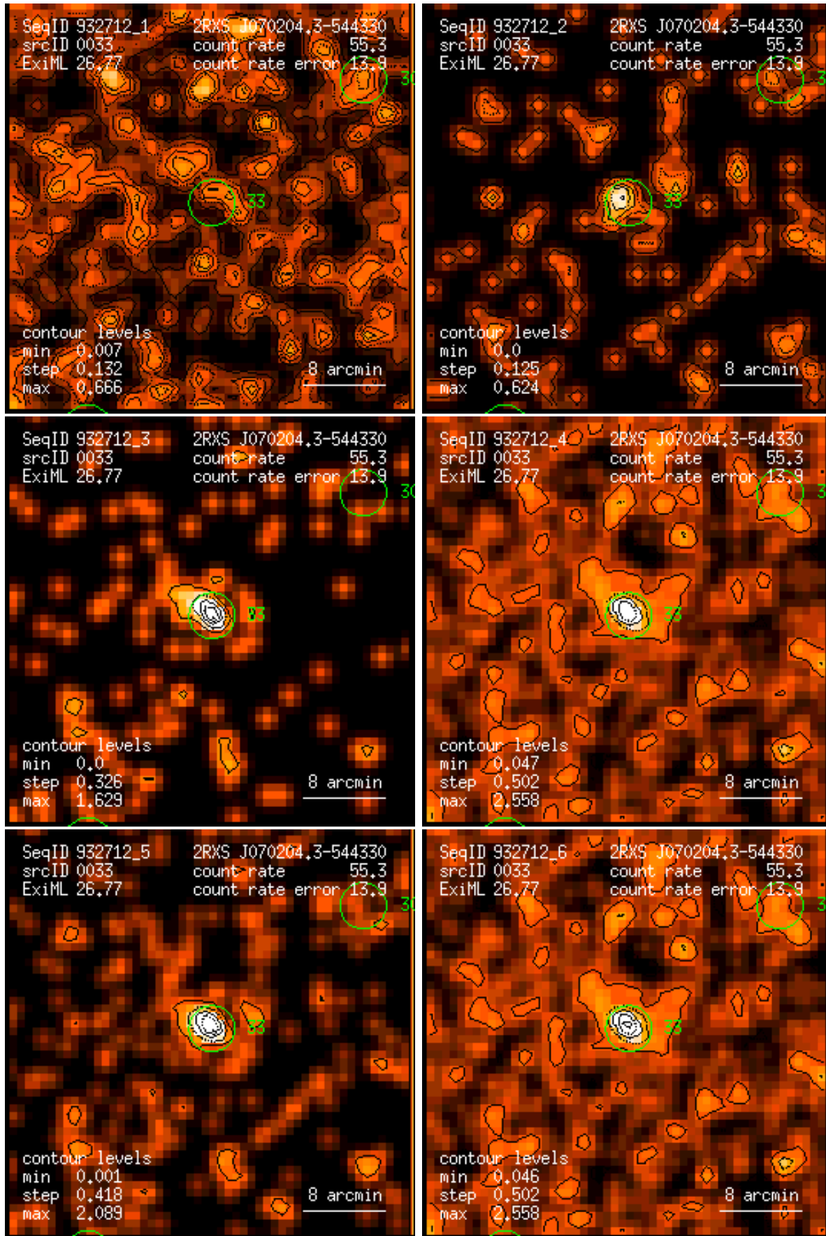
Figure 33: RASS 932712: detection 0033: band rate images, Gaussian filter: (1) PSPC channels 11 – 41, (2) 52 – 90, (3) 91 – 201, (4) 11 – 235, (5) 52 – 201, (6) 11 – 201. Broad band rates in counts/ks. Band rate contour levels in counts/ks/arcmin 2 .
