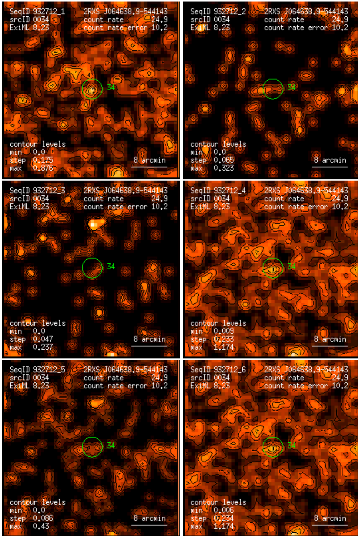
Figure 34: RASS 932712: detection 0034: band rate images, Gaussian filter: (1) PSPC channels 11 – 41, (2) 52 – 90, (3) 91 – 201, (4) 11 – 235, (5) 52 – 201, (6) 11 – 201. Broad band rates in counts/ks. Band rate contour levels in counts/ks/arcmin 2 .
