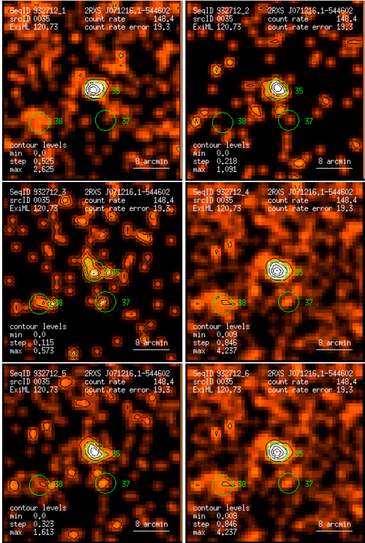
Figure 35: RASS 932712: detection 0035: band rate images, Gaussian filter: (1) PSPC channels 11 – 41, (2) 52 – 90, (3) 91 – 201, (4) 11 – 235, (5) 52 – 201, (6) 11 – 201. Broad band rates in counts/ks. Band rate contour levels in counts/ks/arcmin 2 .
