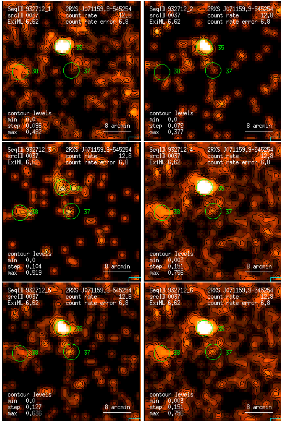
Figure 37: RASS 932712: detection 0037: band rate images, Gaussian filter: (1) PSPC channels 11 – 41, (2) 52 – 90, (3) 91 – 201, (4) 11 – 235, (5) 52 – 201, (6) 11 – 201. Broad band rates in counts/ks. Band rate contour levels in counts/ks/arcmin 2 .
