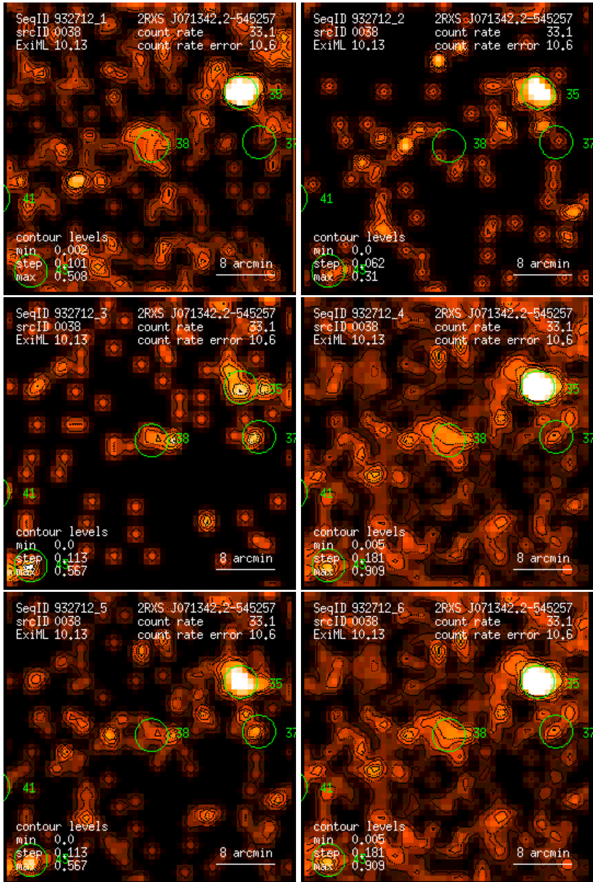
Figure 38: RASS 932712: detection 0038: band rate images, Gaussian filter: (1) PSPC channels 11 – 41, (2) 52 – 90, (3) 91 – 201, (4) 11 – 235, (5) 52 – 201, (6) 11 – 201. Broad band rates in counts/ks. Band rate contour levels in counts/ks/arcmin 2 .
