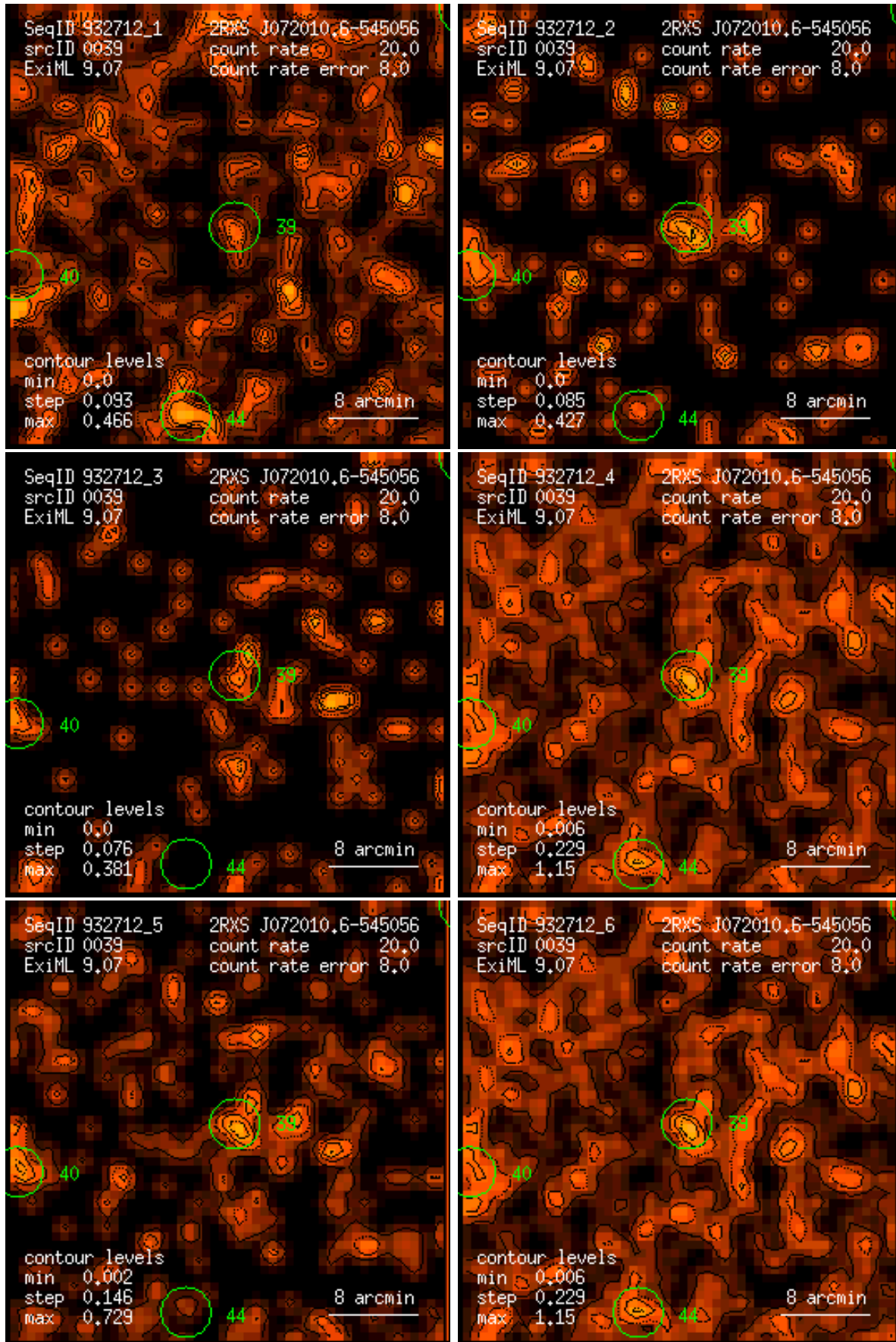
Figure 39: RASS 932712: detection 0039: band rate images, Gaussian filter: (1) PSPC channels 11 – 41, (2) 52 – 90, (3) 91 – 201, (4) 11 – 235, (5) 52 – 201, (6) 11 – 201. Broad band rates in counts/ks. Band rate contour levels in counts/ks/arcmin 2 .
