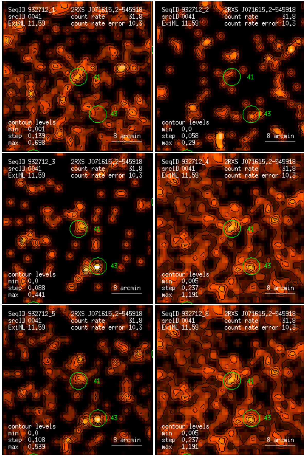
Figure 41: RASS 932712: detection 0041: band rate images, Gaussian filter: (1) PSPC channels 11 – 41, (2) 52 – 90, (3) 91 – 201, (4) 11 – 235, (5) 52 – 201, (6) 11 – 201. Broad band rates in counts/ks. Band rate contour levels in counts/ks/arcmin 2 .
