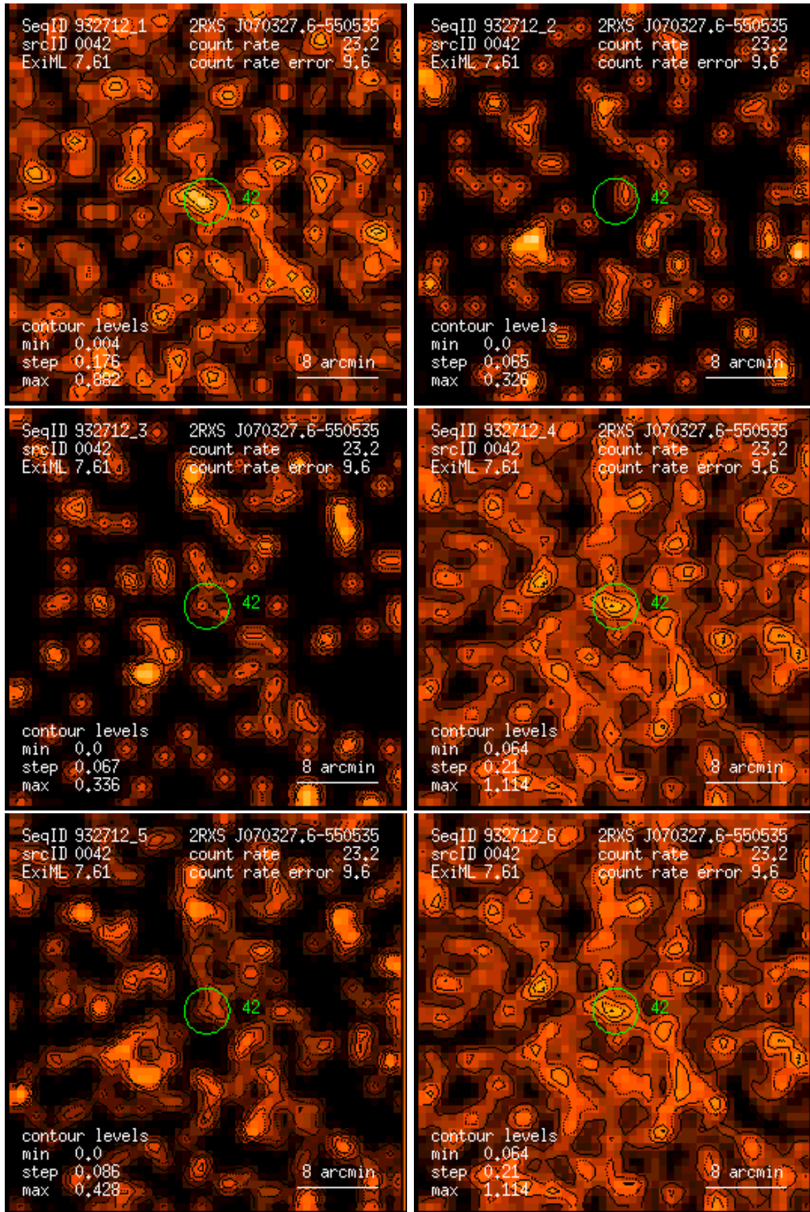
Figure 42: RASS 932712: detection 0042: band rate images, Gaussian filter: (1) PSPC channels 11 – 41, (2) 52 – 90, (3) 91 – 201, (4) 11 – 235, (5) 52 – 201, (6) 11 – 201. Broad band rates in counts/ks. Band rate contour levels in counts/ks/arcmin 2 .
