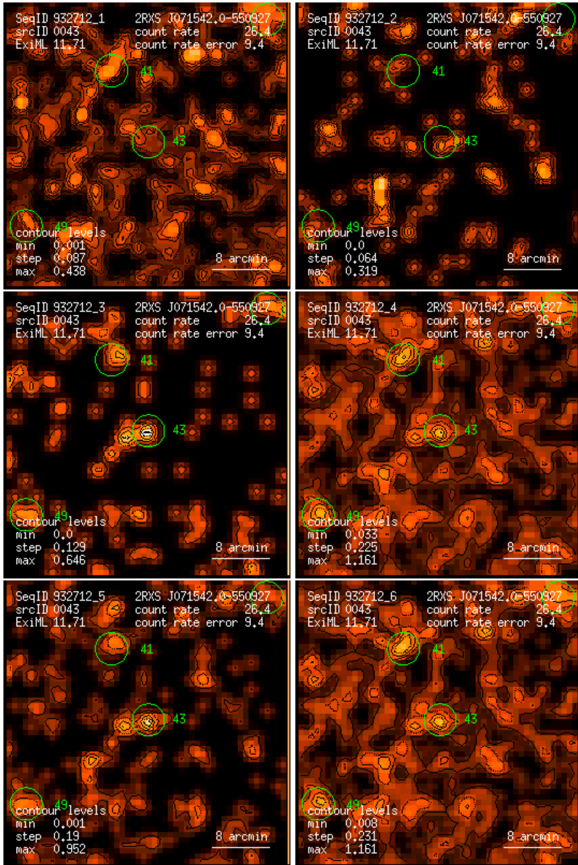
Figure 43: RASS 932712: detection 0043: band rate images, Gaussian filter: (1) PSPC channels 11 – 41, (2) 52 – 90, (3) 91 – 201, (4) 11 – 235, (5) 52 – 201, (6) 11 – 201. Broad band rates in counts/ks. Band rate contour levels in counts/ks/arcmin 2 .
