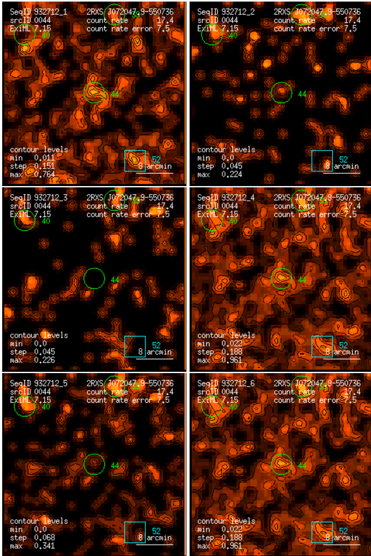
Figure 44: RASS 932712: detection 0044: band rate images, Gaussian filter: (1) PSPC channels 11 – 41, (2) 52 – 90, (3) 91 – 201, (4) 11 – 235, (5) 52 – 201, (6) 11 – 201. Broad band rates in counts/ks. Band rate contour levels in counts/ks/arcmin 2 .
