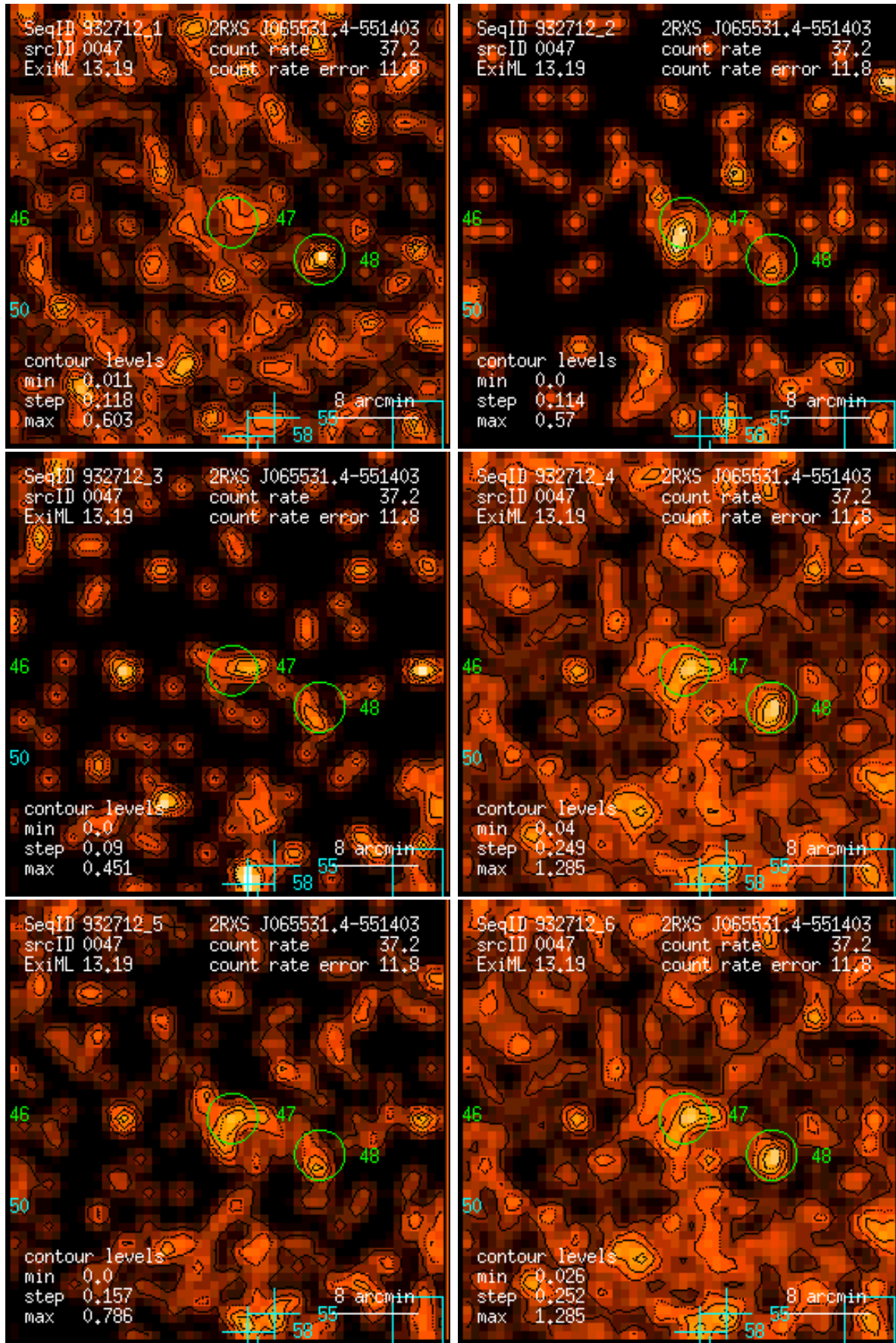
Figure 47: RASS 932712: detection 0047: band rate images, Gaussian filter: (1) PSPC channels 11 – 41, (2) 52 – 90, (3) 91 – 201, (4) 11 – 235, (5) 52 – 201, (6) 11 – 201. Broad band rates in counts/ks. Band rate contour levels in counts/ks/arcmin 2 .
