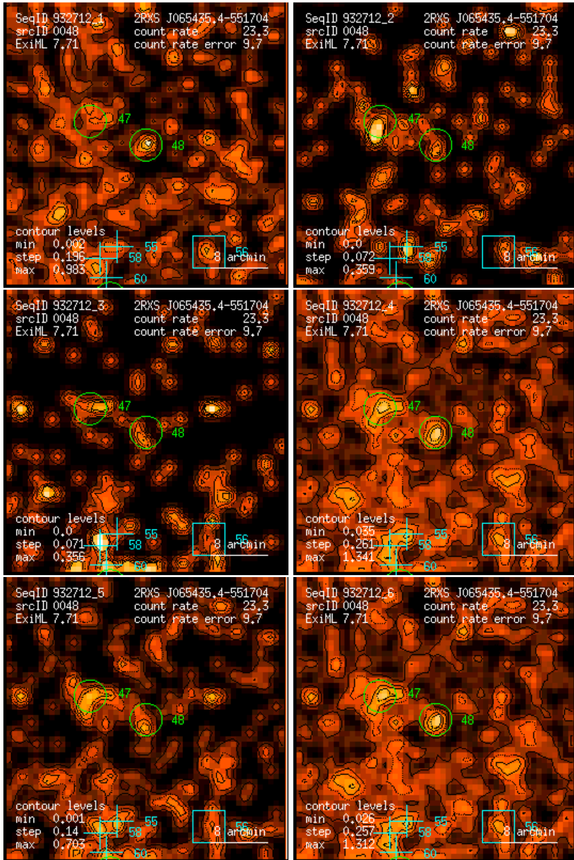
Figure 48: RASS 932712: detection 0048: band rate images, Gaussian filter: (1) PSPC channels 11 – 41, (2) 52 – 90, (3) 91 – 201, (4) 11 – 235, (5) 52 – 201, (6) 11 – 201. Broad band rates in counts/ks. Band rate contour levels in counts/ks/arcmin 2 .
