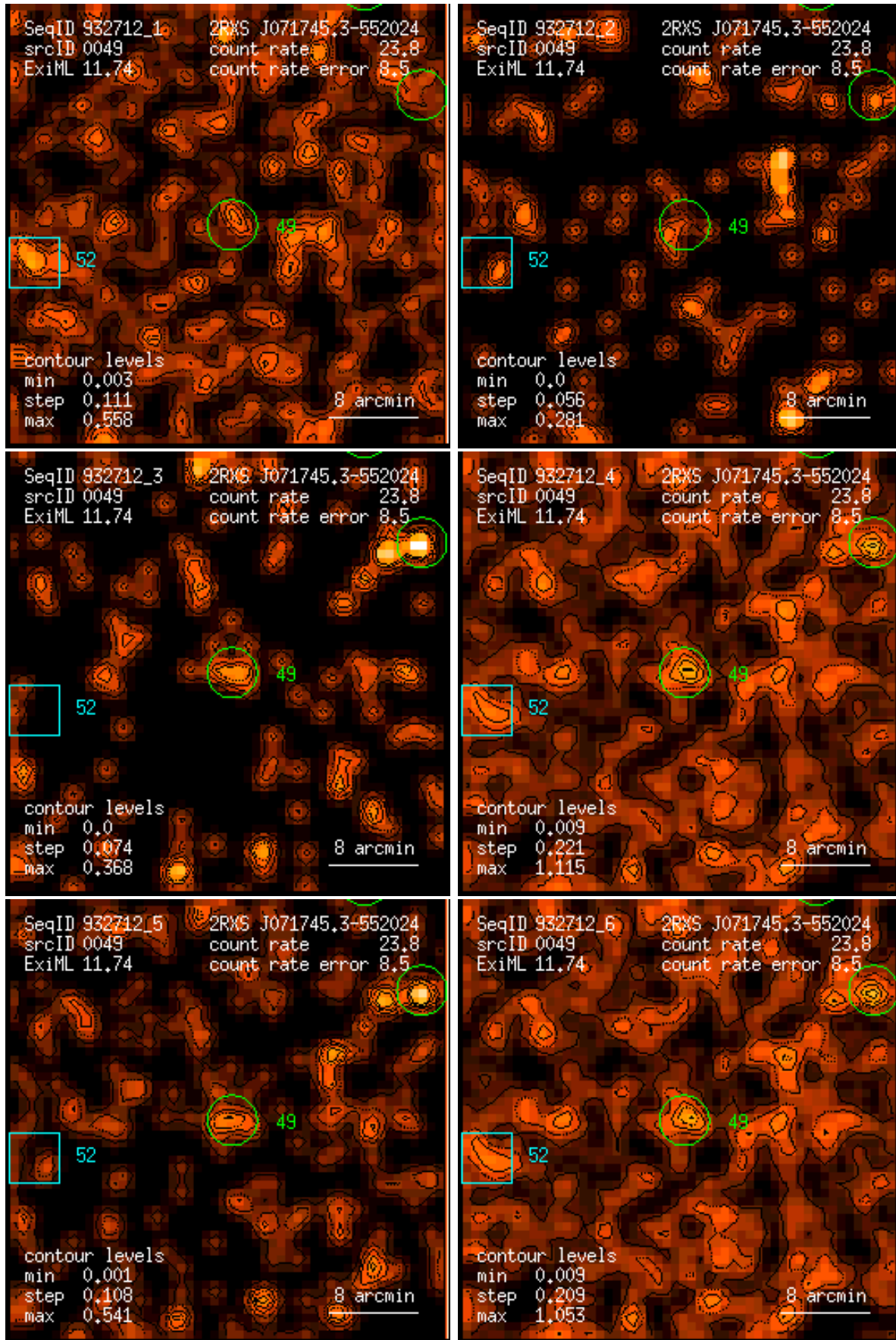
Figure 49: RASS 932712: detection 0049: band rate images, Gaussian filter: (1) PSPC channels 11 – 41, (2) 52 – 90, (3) 91 – 201, (4) 11 – 235, (5) 52 – 201, (6) 11 – 201. Broad band rates in counts/ks. Band rate contour levels in counts/ks/arcmin 2 .
