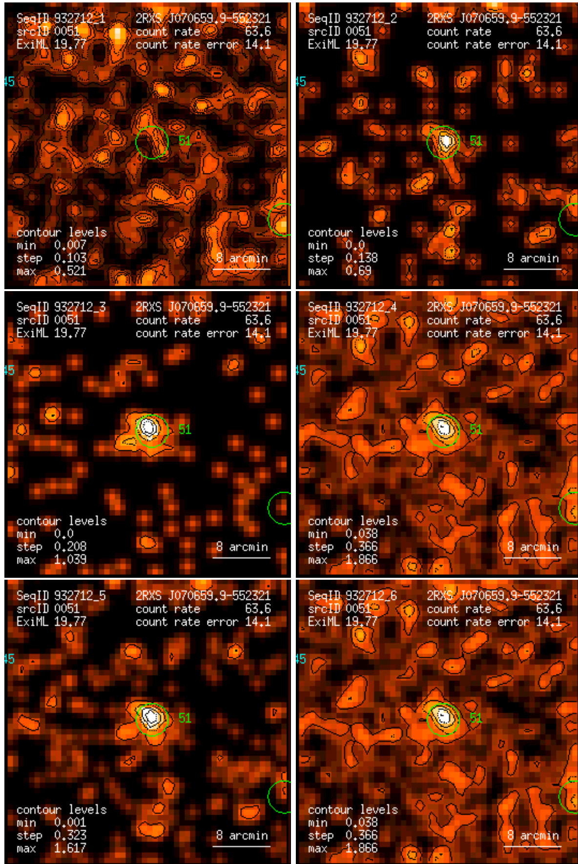
Figure 51: RASS 932712: detection 0051: band rate images, Gaussian filter: (1) PSPC channels 11 – 41, (2) 52 – 90, (3) 91 – 201, (4) 11 – 235, (5) 52 – 201, (6) 11 – 201. Broad band rates in counts/ks. Band rate contour levels in counts/ks/arcmin 2 .
