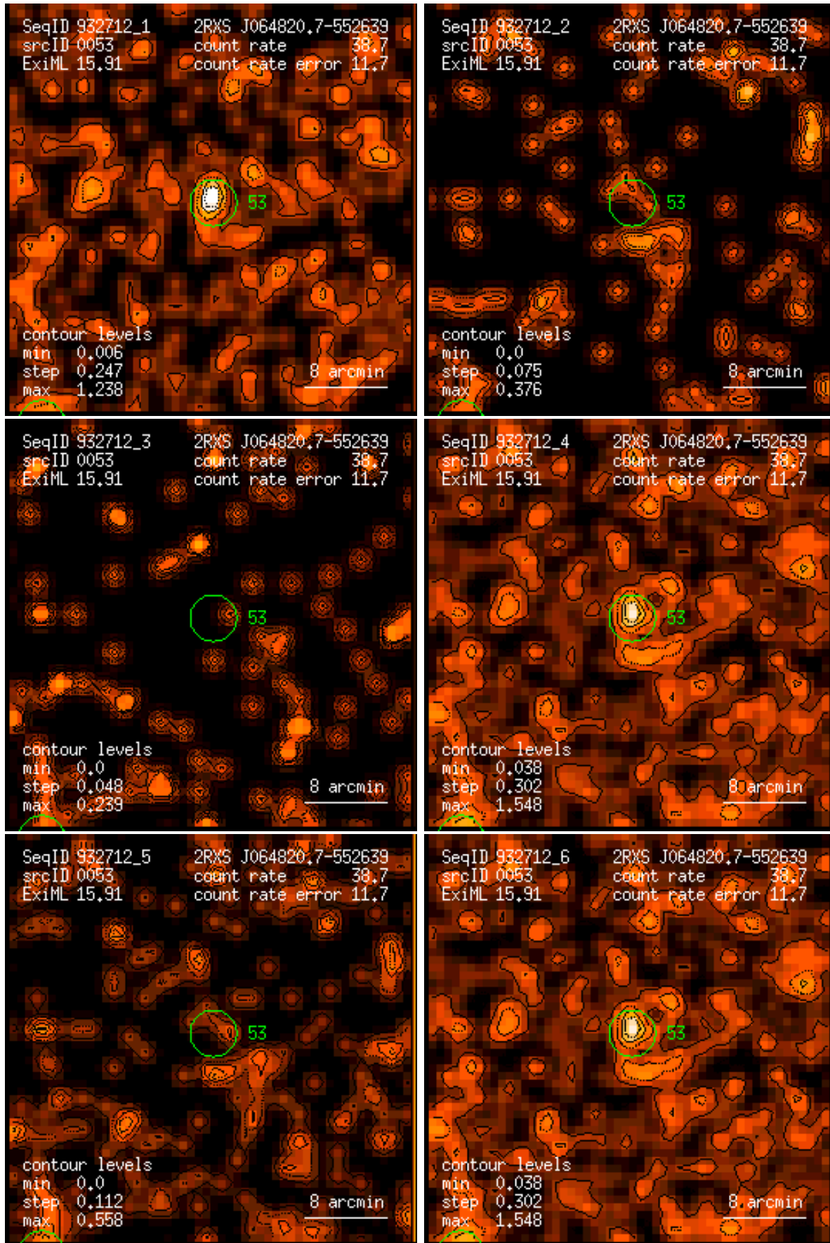
Figure 53: RASS 932712: detection 0053: band rate images, Gaussian filter: (1) PSPC channels 11 – 41, (2) 52 – 90, (3) 91 – 201, (4) 11 – 235, (5) 52 – 201, (6) 11 – 201. Broad band rates in counts/ks. Band rate contour levels in counts/ks/arcmin 2 .
