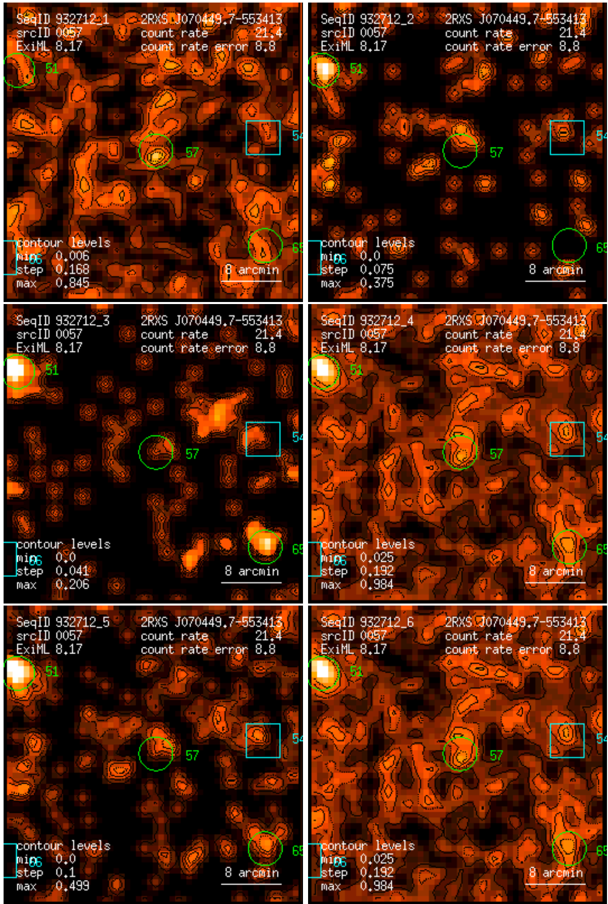
Figure 57: RASS 932712: detection 0057: band rate images, Gaussian filter: (1) PSPC channels 11 – 41, (2) 52 – 90, (3) 91 – 201, (4) 11 – 235, (5) 52 – 201, (6) 11 – 201. Broad band rates in counts/ks. Band rate contour levels in counts/ks/arcmin 2 .
