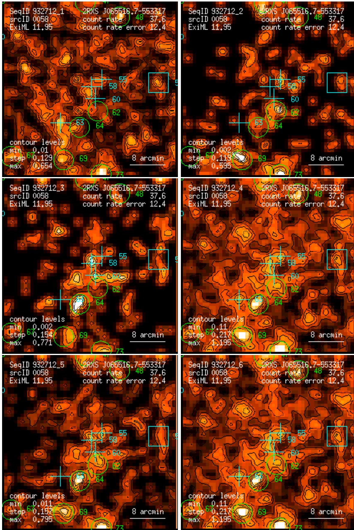
Figure 58: RASS 932712: detection 0058: band rate images, Gaussian filter: (1) PSPC channels 11 – 41, (2) 52 – 90, (3) 91 – 201, (4) 11 – 235, (5) 52 – 201, (6) 11 – 201. Broad band rates in counts/ks. Band rate contour levels in counts/ks/arcmin 2 .
