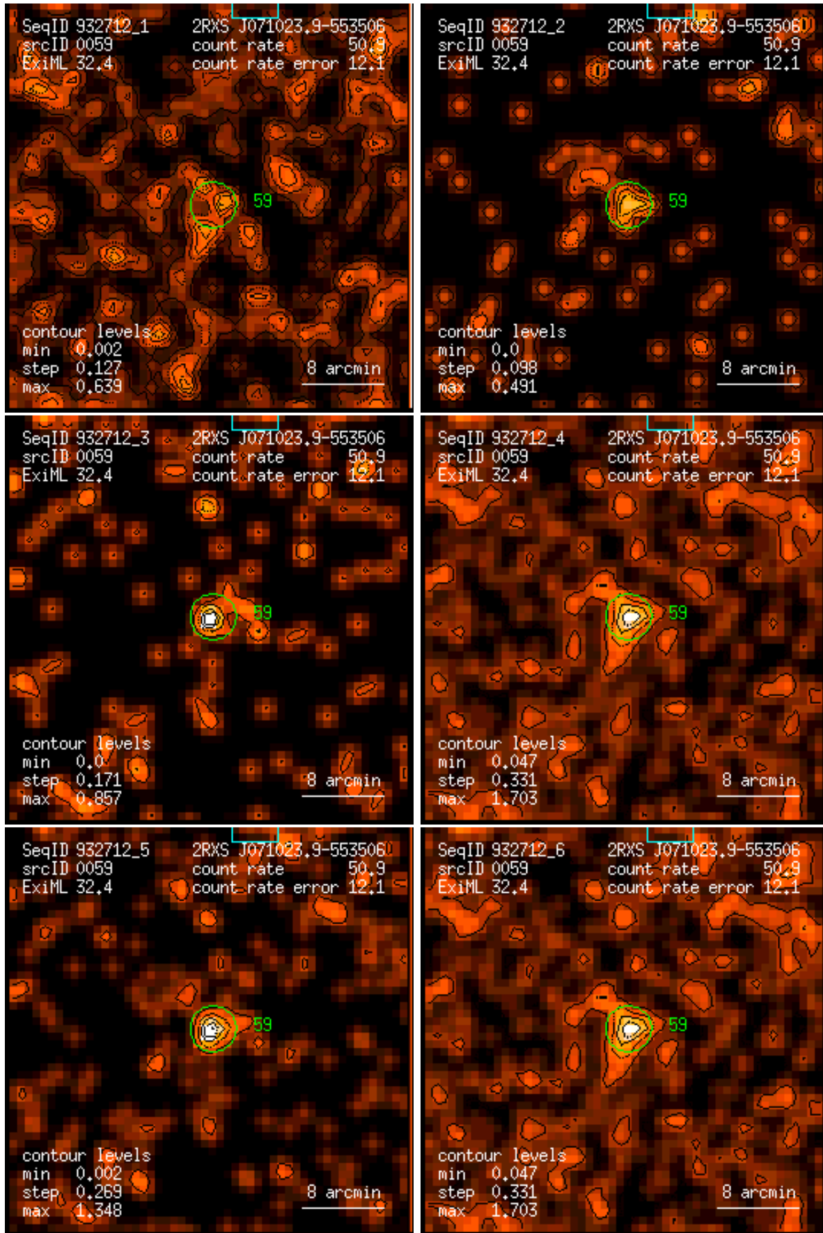
Figure 59: RASS 932712: detection 0059: band rate images, Gaussian filter: (1) PSPC channels 11 – 41, (2) 52 – 90, (3) 91 – 201, (4) 11 – 235, (5) 52 – 201, (6) 11 – 201. Broad band rates in counts/ks. Band rate contour levels in counts/ks/arcmin 2 .
