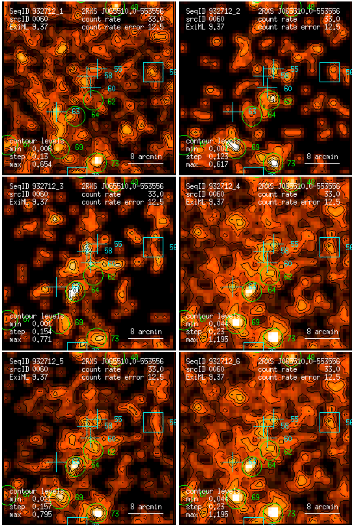
Figure 60: RASS 932712: detection 0060: band rate images, Gaussian filter: (1) PSPC channels 11 – 41, (2) 52 – 90, (3) 91 – 201, (4) 11 – 235, (5) 52 – 201, (6) 11 – 201. Broad band rates in counts/ks. Band rate contour levels in counts/ks/arcmin 2 .
