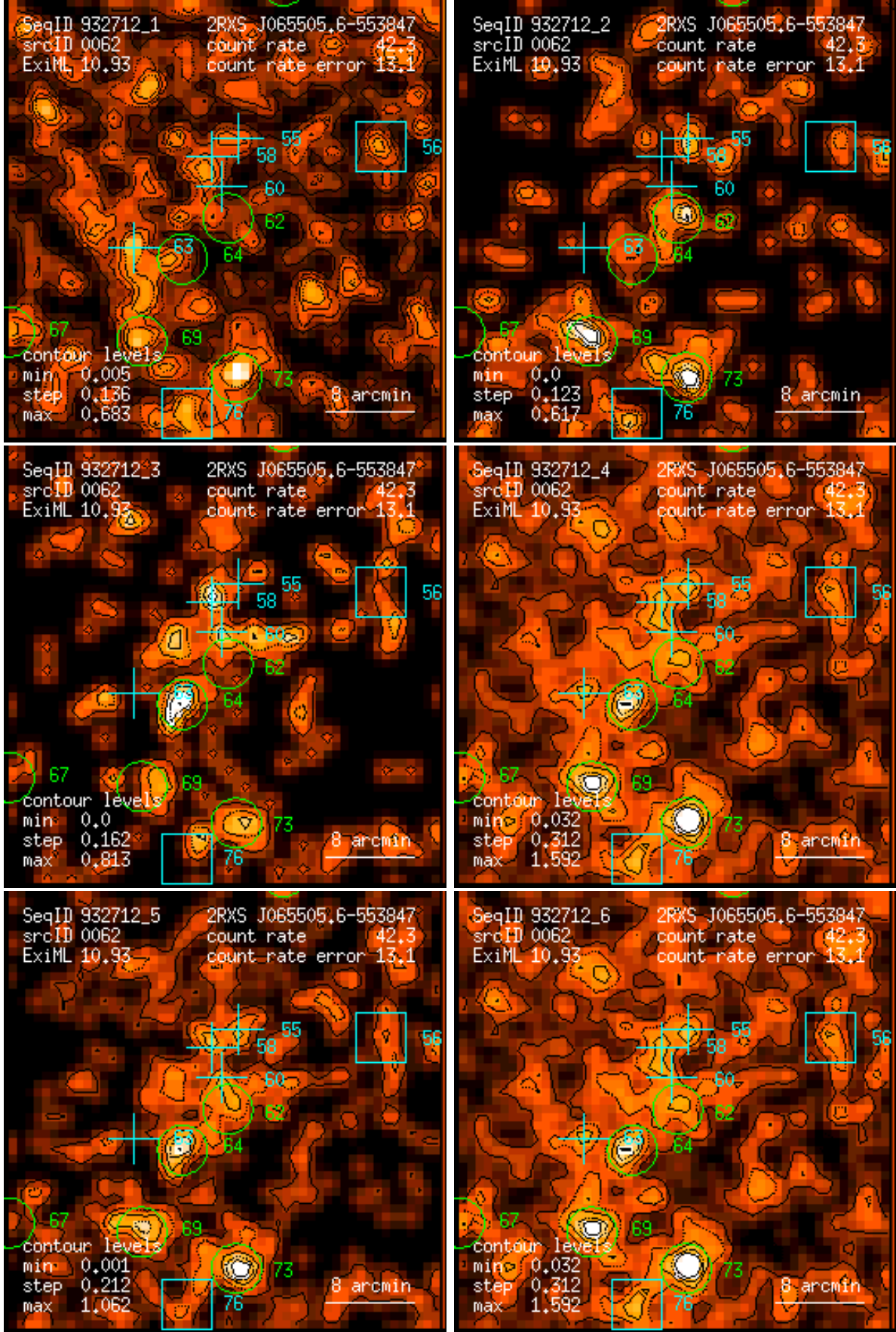
Figure 62: RASS 932712: detection 0062: band rate images, Gaussian filter: (1) PSPC channels 11 – 41, (2) 52 – 90, (3) 91 – 201, (4) 11 – 235, (5) 52 – 201, (6) 11 – 201. Broad band rates in counts/ks. Band rate contour levels in counts/ks/arcmin 2 .
