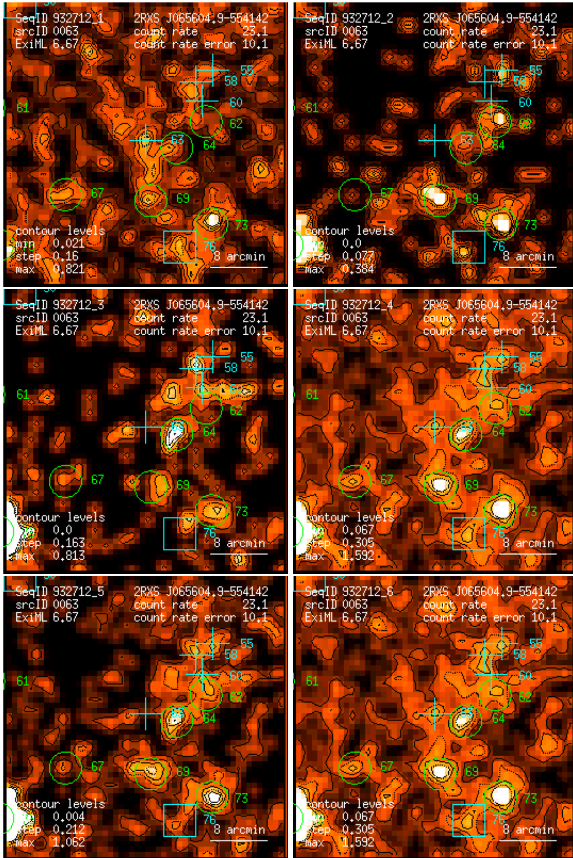
Figure 63: RASS 932712: detection 0063: band rate images, Gaussian filter: (1) PSPC channels 11 – 41, (2) 52 – 90, (3) 91 – 201, (4) 11 – 235, (5) 52 – 201, (6) 11 – 201. Broad band rates in counts/ks. Band rate contour levels in counts/ks/arcmin 2 .
