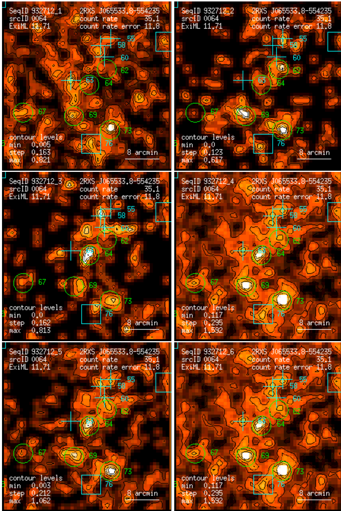
Figure 64: RASS 932712: detection 0064: band rate images, Gaussian filter: (1) PSPC channels 11 – 41, (2) 52 – 90, (3) 91 – 201, (4) 11 – 235, (5) 52 – 201, (6) 11 – 201. Broad band rates in counts/ks. Band rate contour levels in counts/ks/arcmin 2 .
