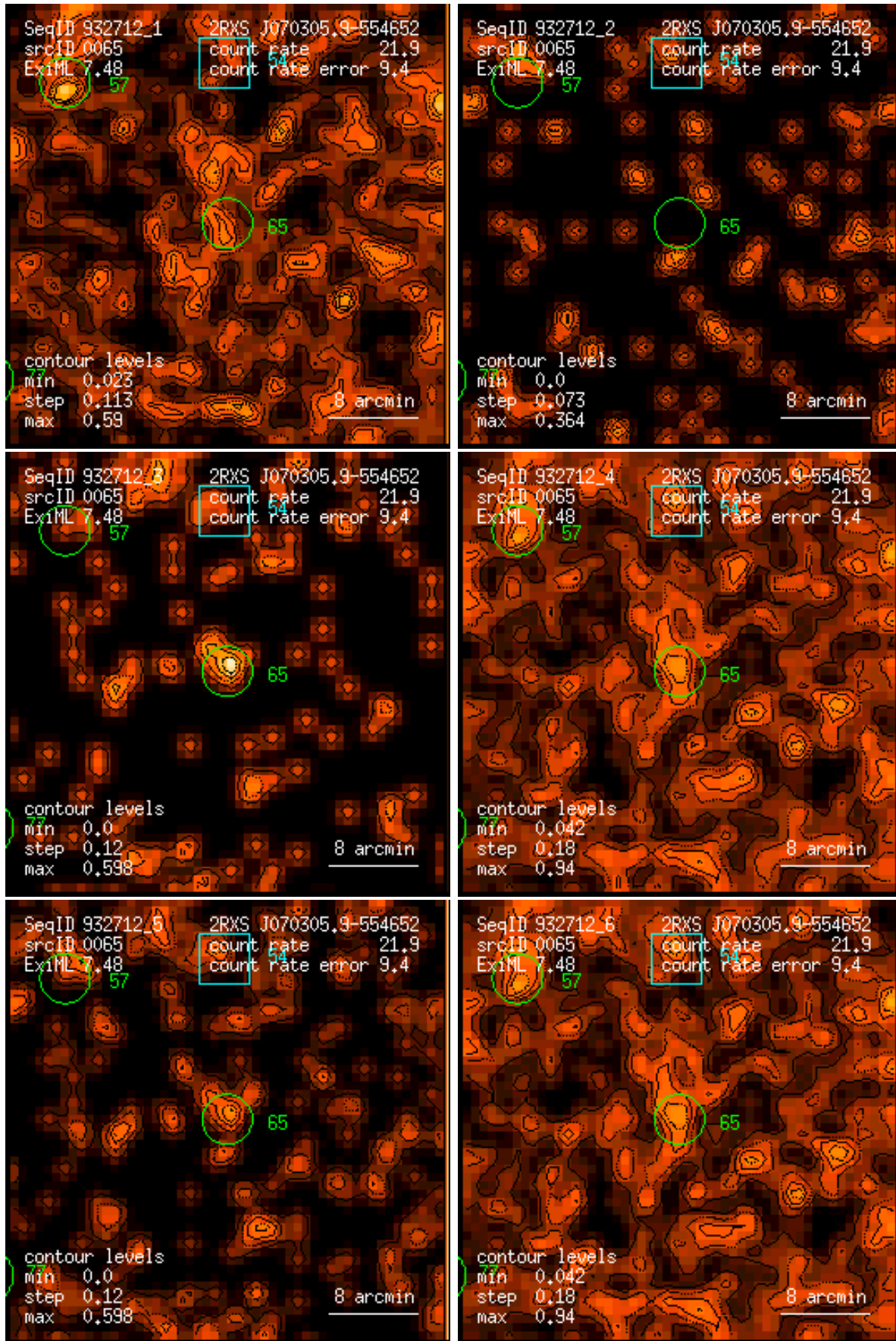
Figure 65: RASS 932712: detection 0065: band rate images, Gaussian filter: (1) PSPC channels 11 – 41, (2) 52 – 90, (3) 91 – 201, (4) 11 – 235, (5) 52 – 201, (6) 11 – 201. Broad band rates in counts/ks. Band rate contour levels in counts/ks/arcmin 2 .
