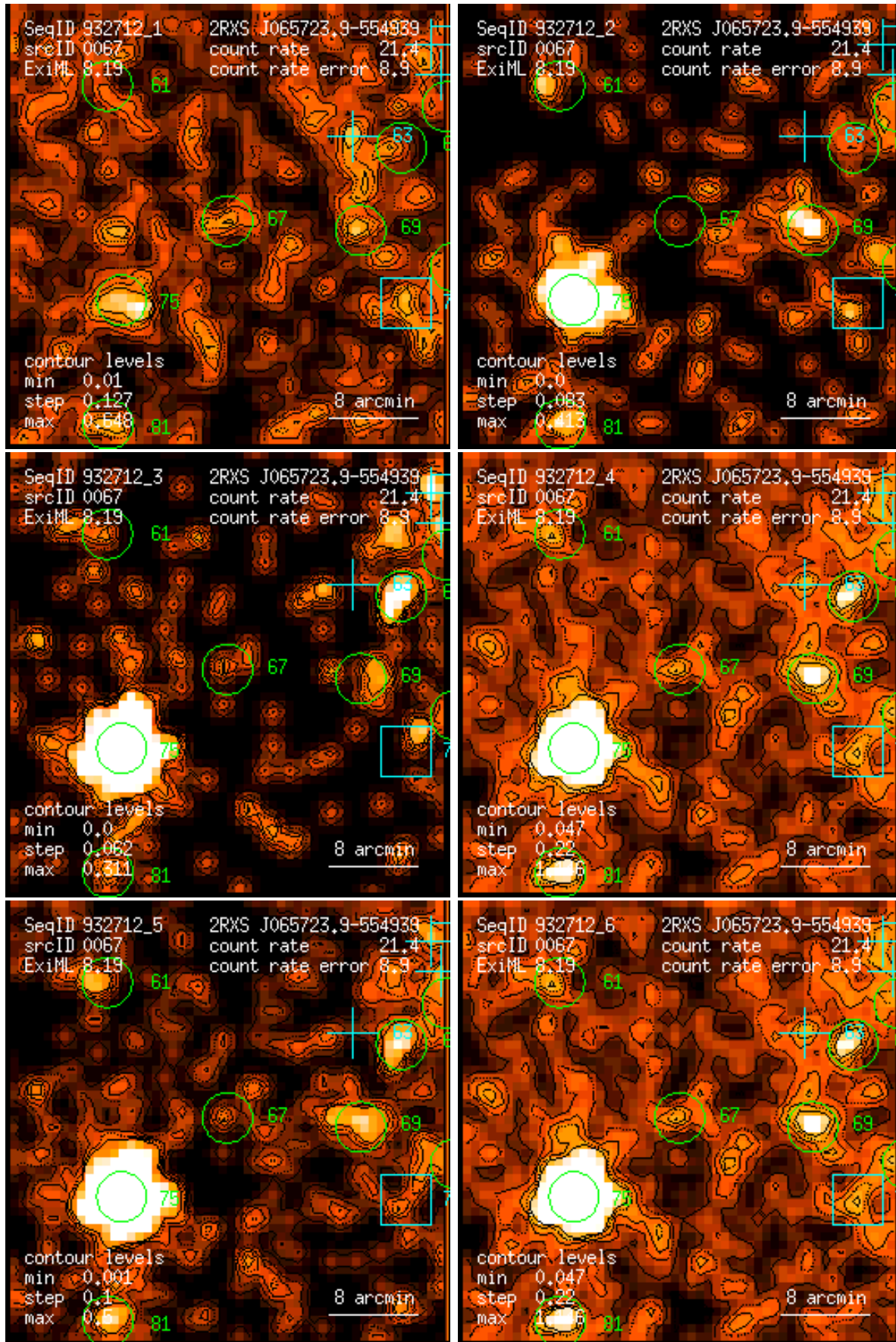
Figure 67: RASS 932712: detection 0067: band rate images, Gaussian filter: (1) PSPC channels 11 – 41, (2) 52 – 90, (3) 91 – 201, (4) 11 – 235, (5) 52 – 201, (6) 11 – 201. Broad band rates in counts/ks. Band rate contour levels in counts/ks/arcmin 2 .
