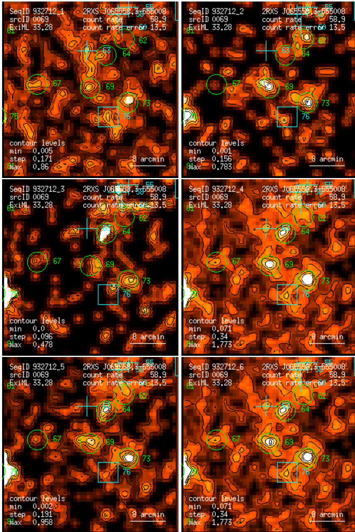
Figure 69: RASS 932712: detection 0069: band rate images, Gaussian filter: (1) PSPC channels 11 – 41, (2) 52 – 90, (3) 91 – 201, (4) 11 – 235, (5) 52 – 201, (6) 11 – 201. Broad band rates in counts/ks. Band rate contour levels in counts/ks/arcmin 2 .
