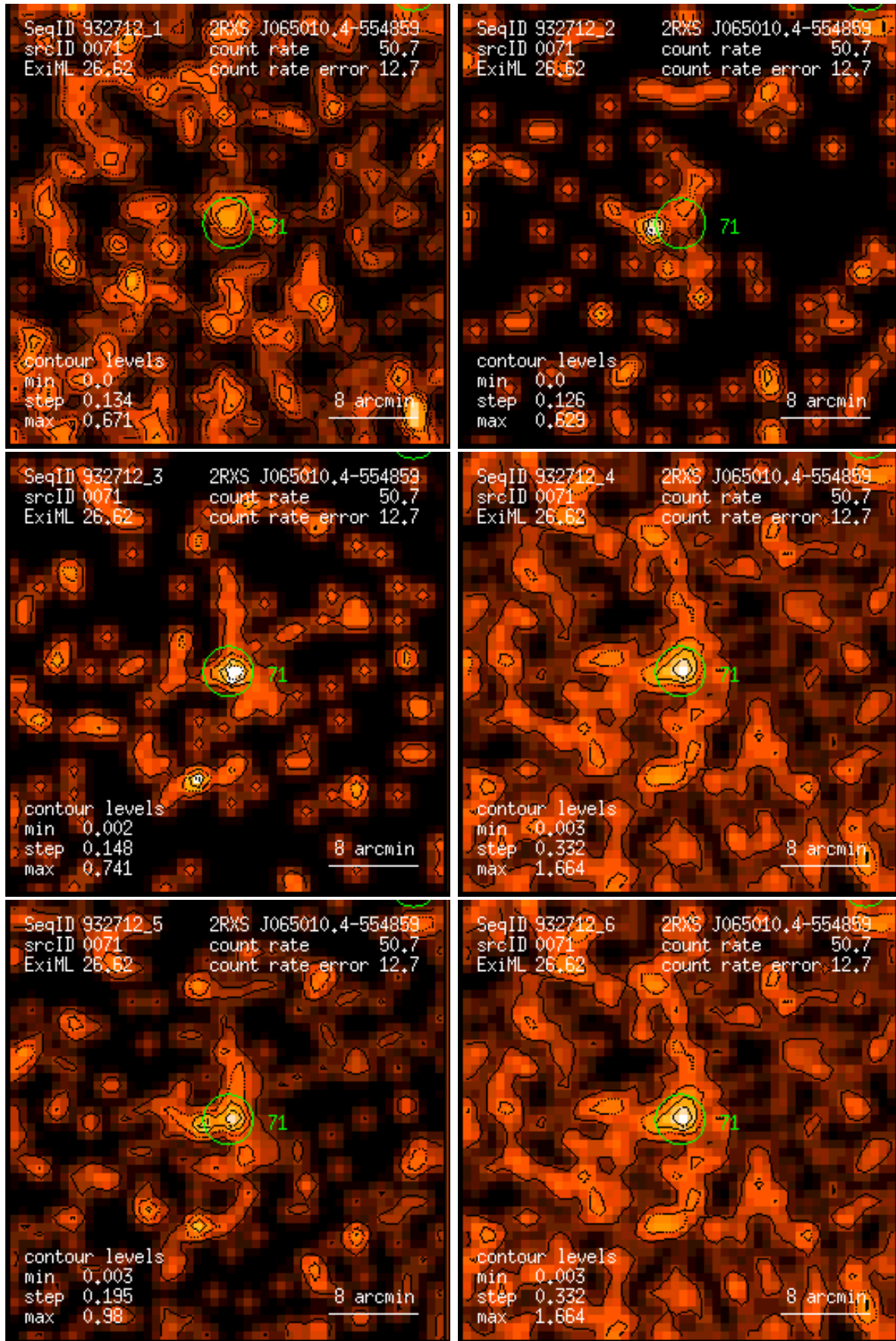
Figure 71: RASS 932712: detection 0071: band rate images, Gaussian filter: (1) PSPC channels 11 – 41, (2) 52 – 90, (3) 91 – 201, (4) 11 – 235, (5) 52 – 201, (6) 11 – 201. Broad band rates in counts/ks. Band rate contour levels in counts/ks/arcmin 2 .
