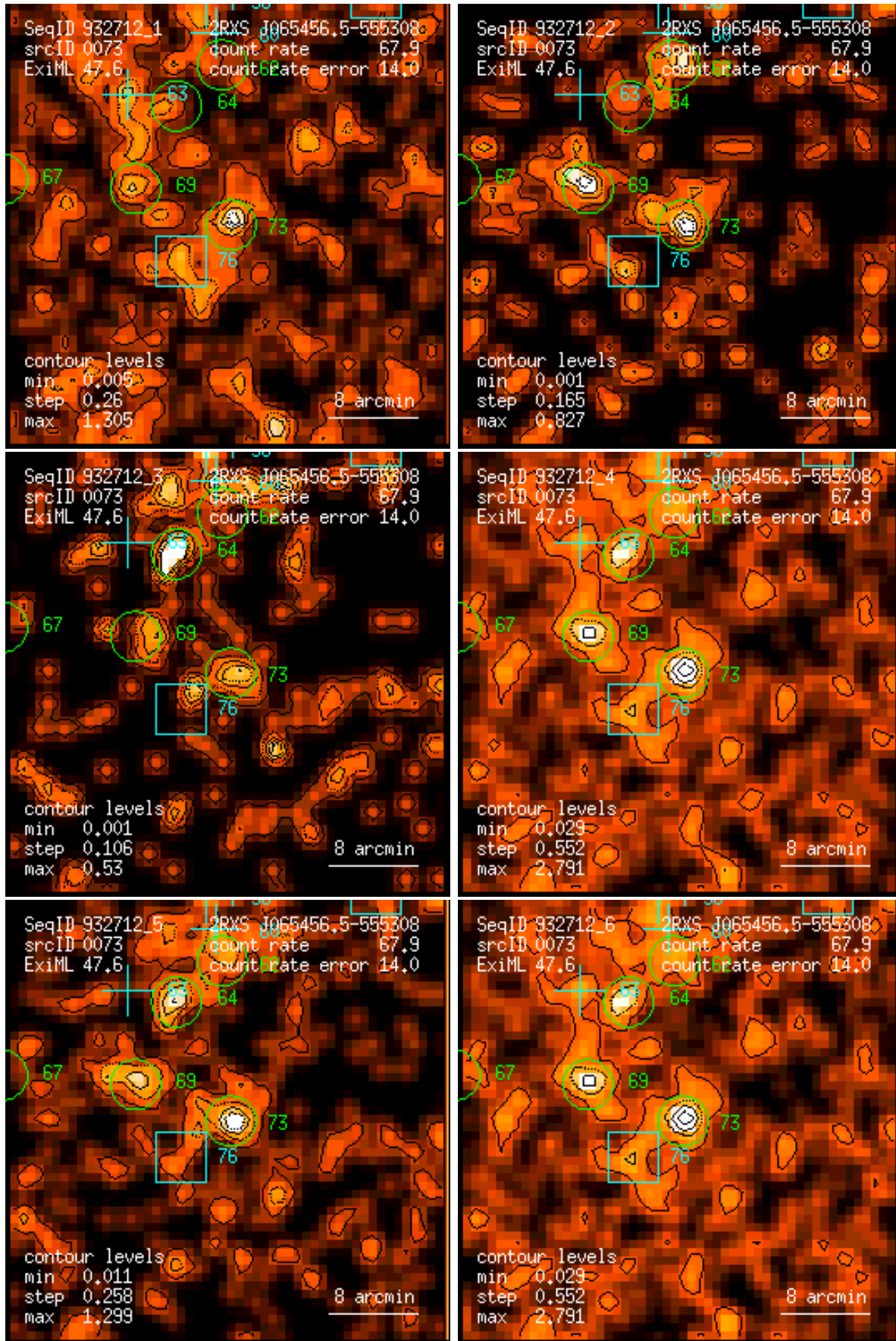
Figure 73: RASS 932712: detection 0073: band rate images, Gaussian filter: (1) PSPC channels 11 – 41, (2) 52 – 90, (3) 91 – 201, (4) 11 – 235, (5) 52 – 201, (6) 11 – 201. Broad band rates in counts/ks. Band rate contour levels in counts/ks/arcmin 2 .
