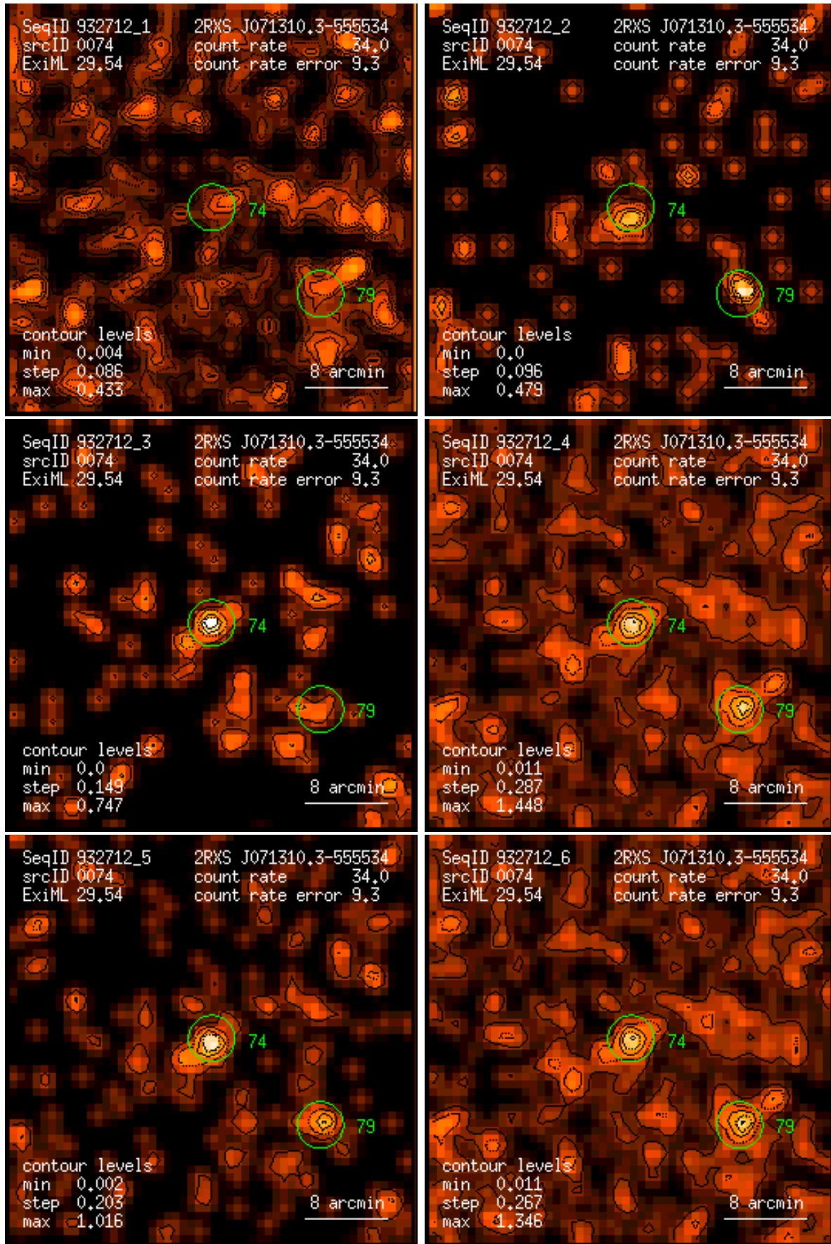
Figure 74: RASS 932712: detection 0074: band rate images, Gaussian filter: (1) PSPC channels 11 – 41, (2) 52 – 90, (3) 91 – 201, (4) 11 – 235, (5) 52 – 201, (6) 11 – 201. Broad band rates in counts/ks. Band rate contour levels in counts/ks/arcmin 2 .
