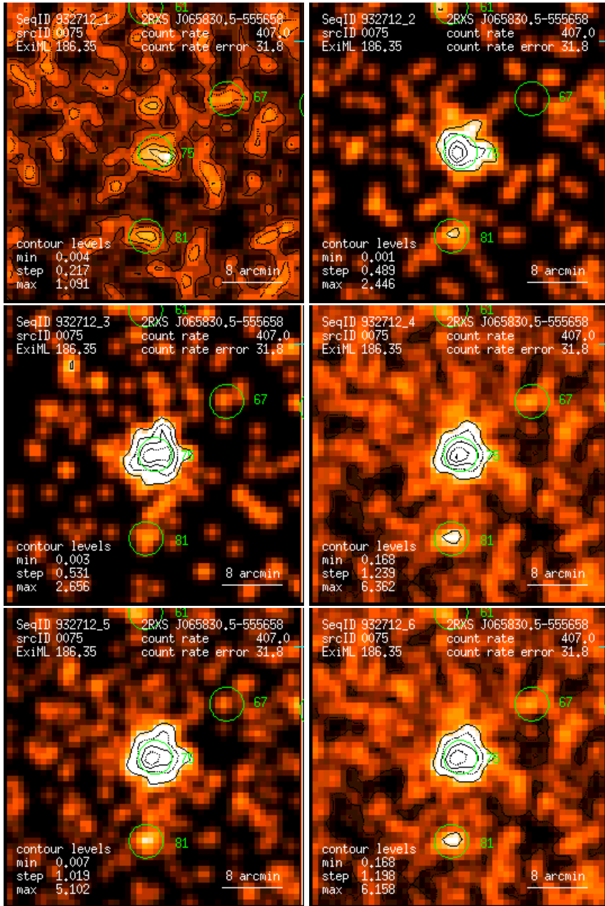
Figure 75: RASS 932712: detection 0075: band rate images, Gaussian filter: (1) PSPC channels 11 – 41, (2) 52 – 90, (3) 91 – 201, (4) 11 – 235, (5) 52 – 201, (6) 11 – 201. Broad band rates in counts/ks. Band rate contour levels in counts/ks/arcmin 2 .
